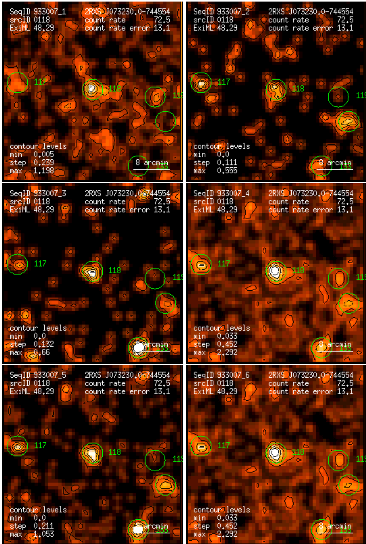
Figure 118: RASS 933007: detection 0118: band rate images, Gaussian filter: (1) PSPC channels 11 – 41, (2) 52 – 90, (3) 91 – 201, (4) 11 – 235, (5) 52 – 201, (6) 11 – 201. Broad band rates in counts/ks. Band rate contour levels in counts/ks/arcmin 2 .
