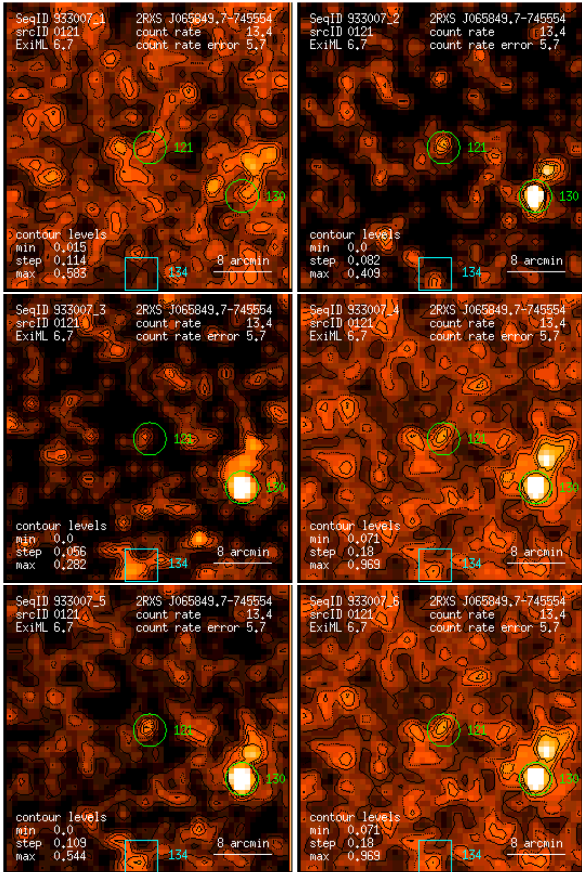
Figure 121: RASS 933007: detection 0121: band rate images, Gaussian filter: (1) PSPC channels 11 – 41, (2) 52 – 90, (3) 91 – 201, (4) 11 – 235, (5) 52 – 201, (6) 11 – 201. Broad band rates in counts/ks. Band rate contour levels in counts/ks/arcmin 2 .
