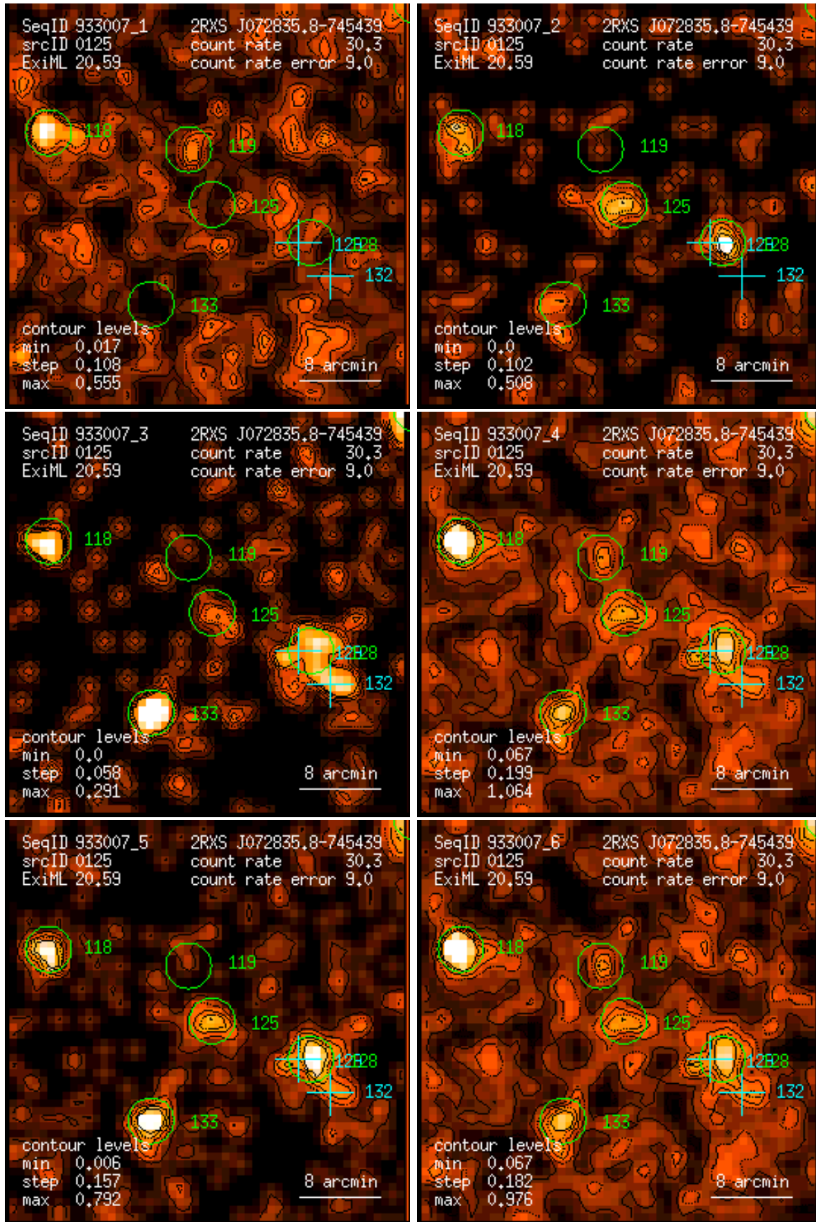
Figure 125: RASS 933007: detection 0125: band rate images, Gaussian filter: (1) PSPC channels 11 – 41, (2) 52 – 90, (3) 91 – 201, (4) 11 – 235, (5) 52 – 201, (6) 11 – 201. Broad band rates in counts/ks. Band rate contour levels in counts/ks/arcmin 2 .
