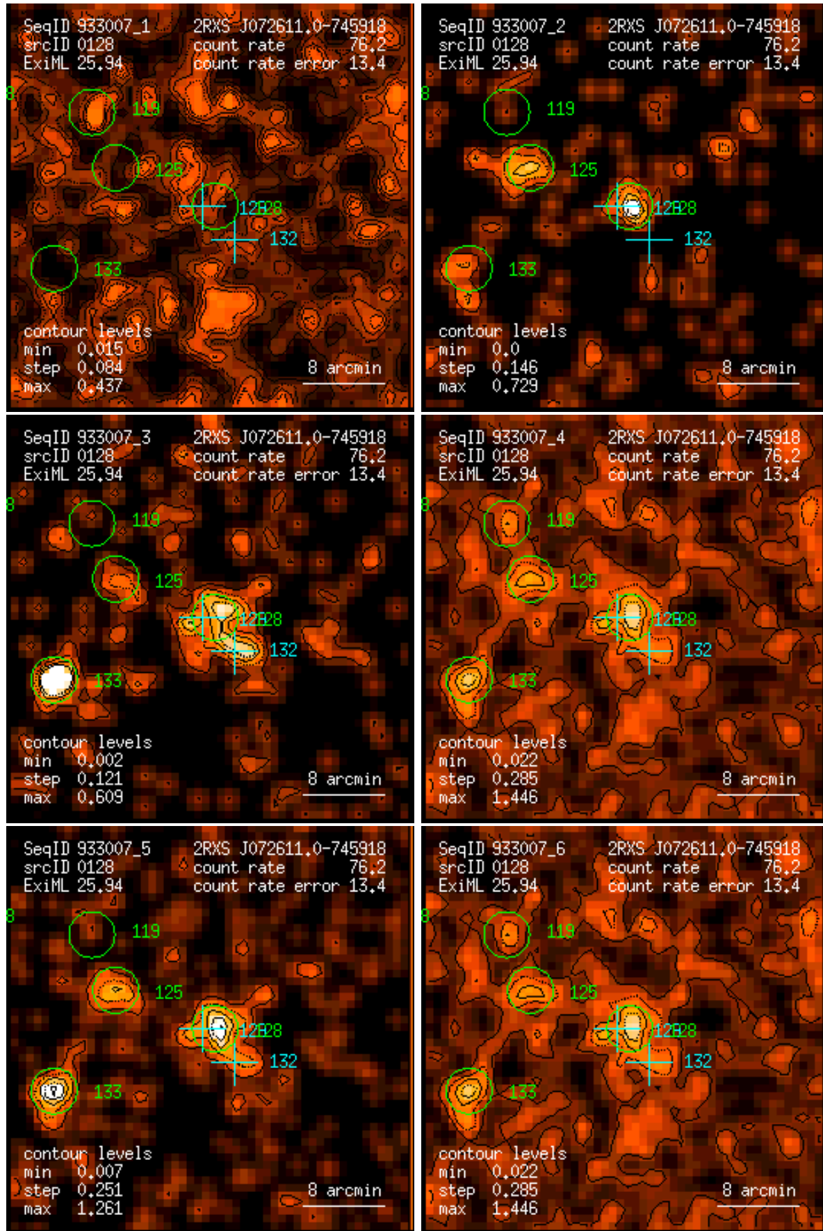
Figure 128: RASS 933007: detection 0128: band rate images, Gaussian filter: (1) PSPC channels 11 – 41, (2) 52 – 90, (3) 91 – 201, (4) 11 – 235, (5) 52 – 201, (6) 11 – 201. Broad band rates in counts/ks. Band rate contour levels in counts/ks/arcmin 2 .
