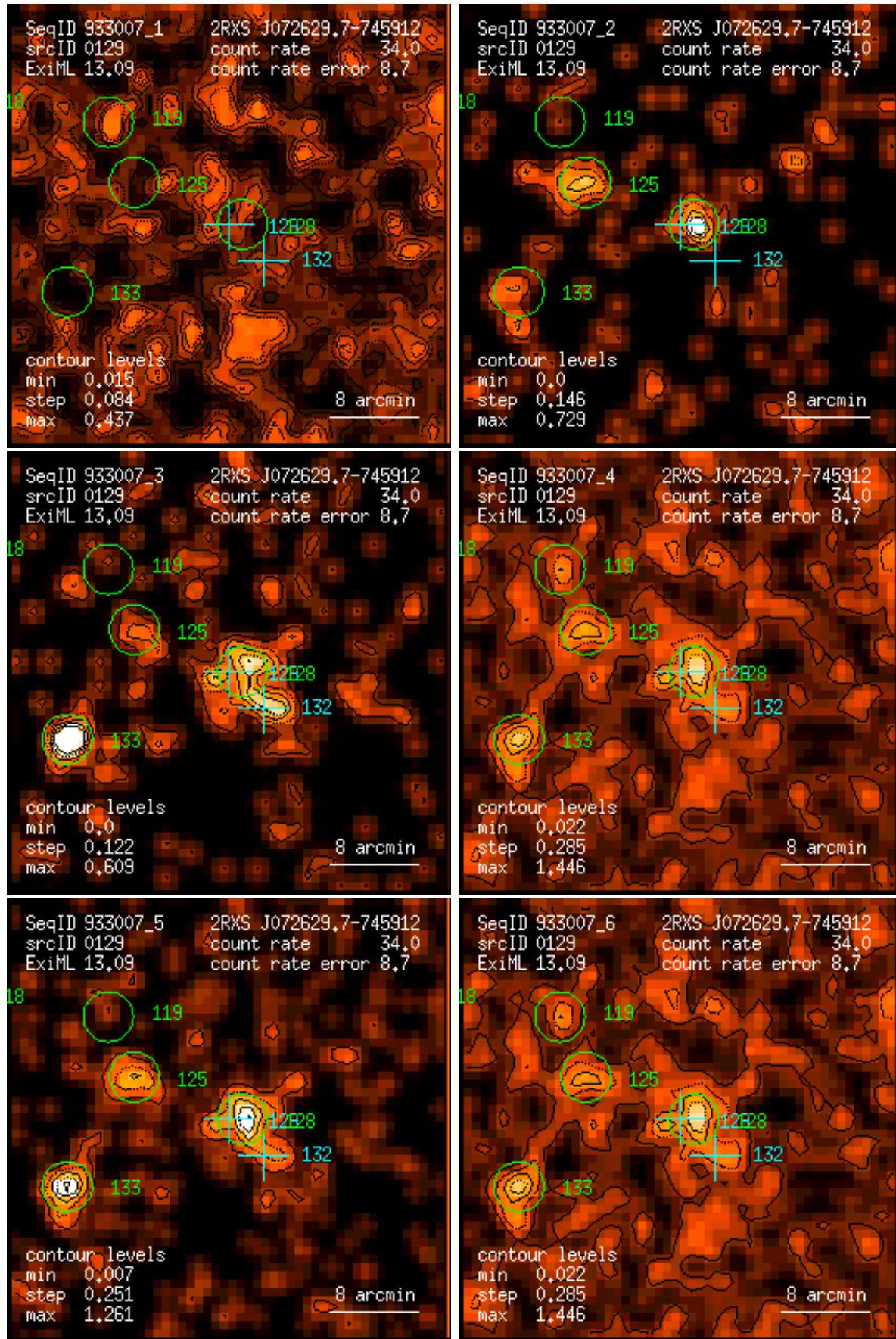
Figure 129: RASS 933007: detection 0129: band rate images, Gaussian filter: (1) PSPC channels 11 – 41, (2) 52 – 90, (3) 91 – 201, (4) 11 – 235, (5) 52 – 201, (6) 11 – 201. Broad band rates in counts/ks. Band rate contour levels in counts/ks/arcmin 2 .
