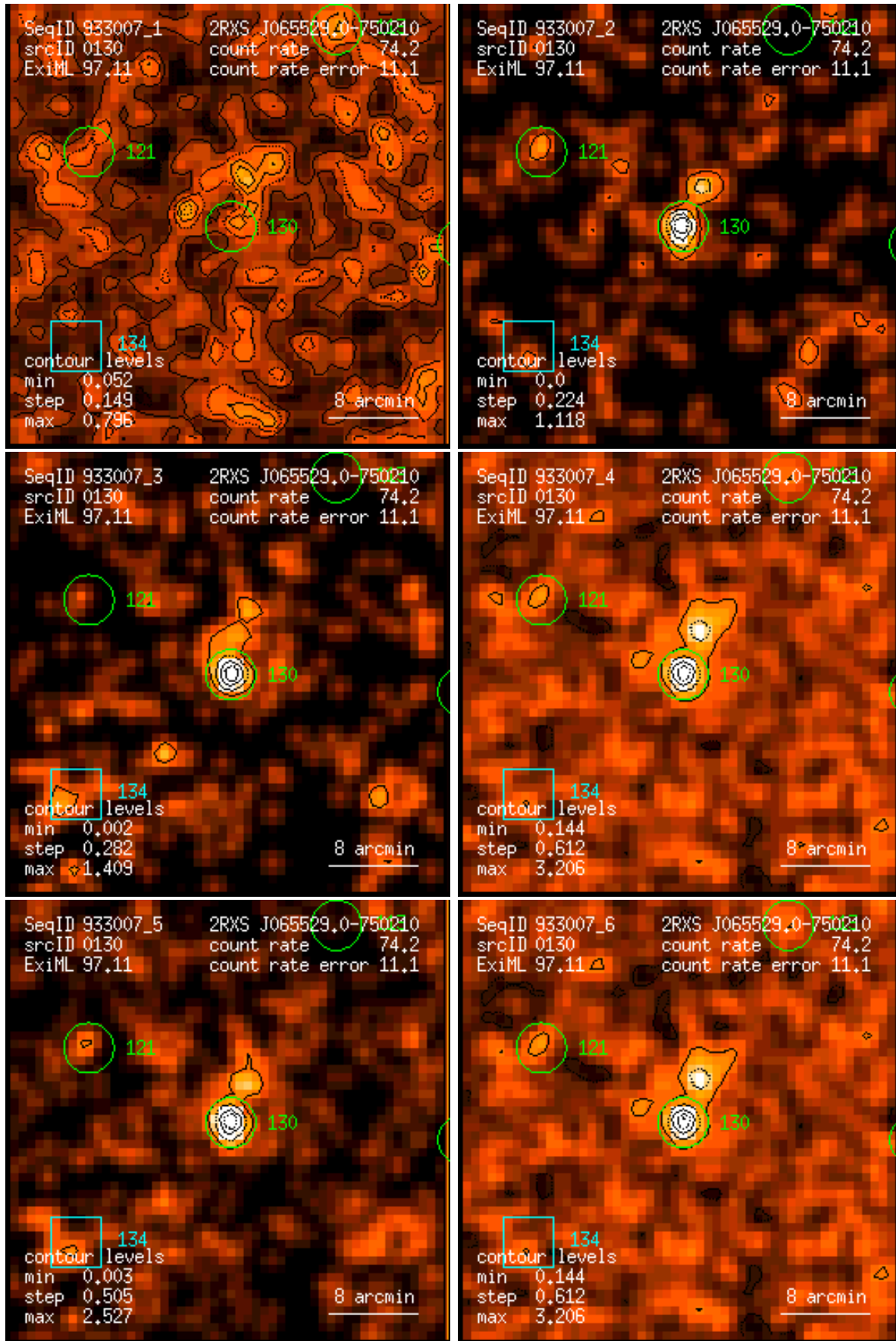
Figure 130: RASS 933007: detection 0130: band rate images, Gaussian filter: (1) PSPC channels 11 – 41, (2) 52 – 90, (3) 91 – 201, (4) 11 – 235, (5) 52 – 201, (6) 11 – 201. Broad band rates in counts/ks. Band rate contour levels in counts/ks/arcmin 2 .
