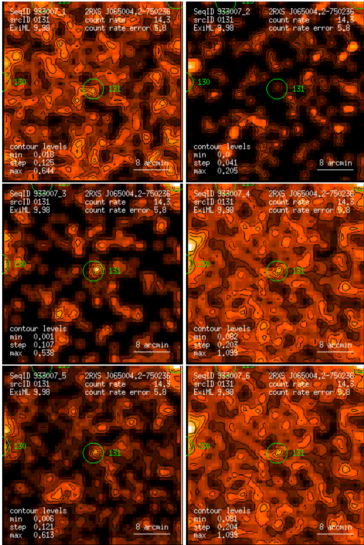
Figure 131: RASS 933007: detection 0131: band rate images, Gaussian filter: (1) PSPC channels 11 – 41, (2) 52 – 90, (3) 91 – 201, (4) 11 – 235, (5) 52 – 201, (6) 11 – 201. Broad band rates in counts/ks. Band rate contour levels in counts/ks/arcmin 2 .
