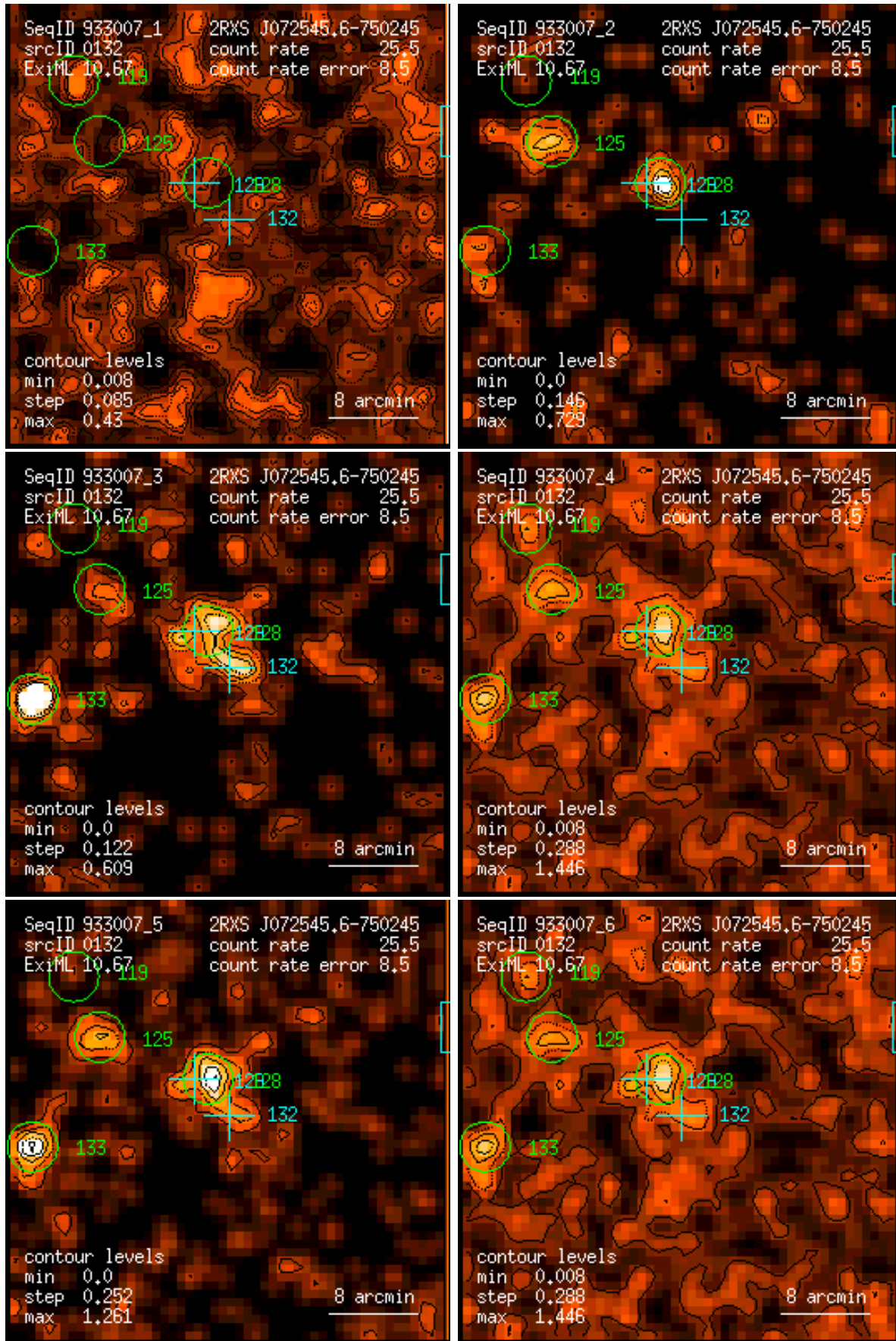
Figure 132: RASS 933007: detection 0132: band rate images, Gaussian filter: (1) PSPC channels 11 – 41, (2) 52 – 90, (3) 91 – 201, (4) 11 – 235, (5) 52 – 201, (6) 11 – 201. Broad band rates in counts/ks. Band rate contour levels in counts/ks/arcmin 2 .
