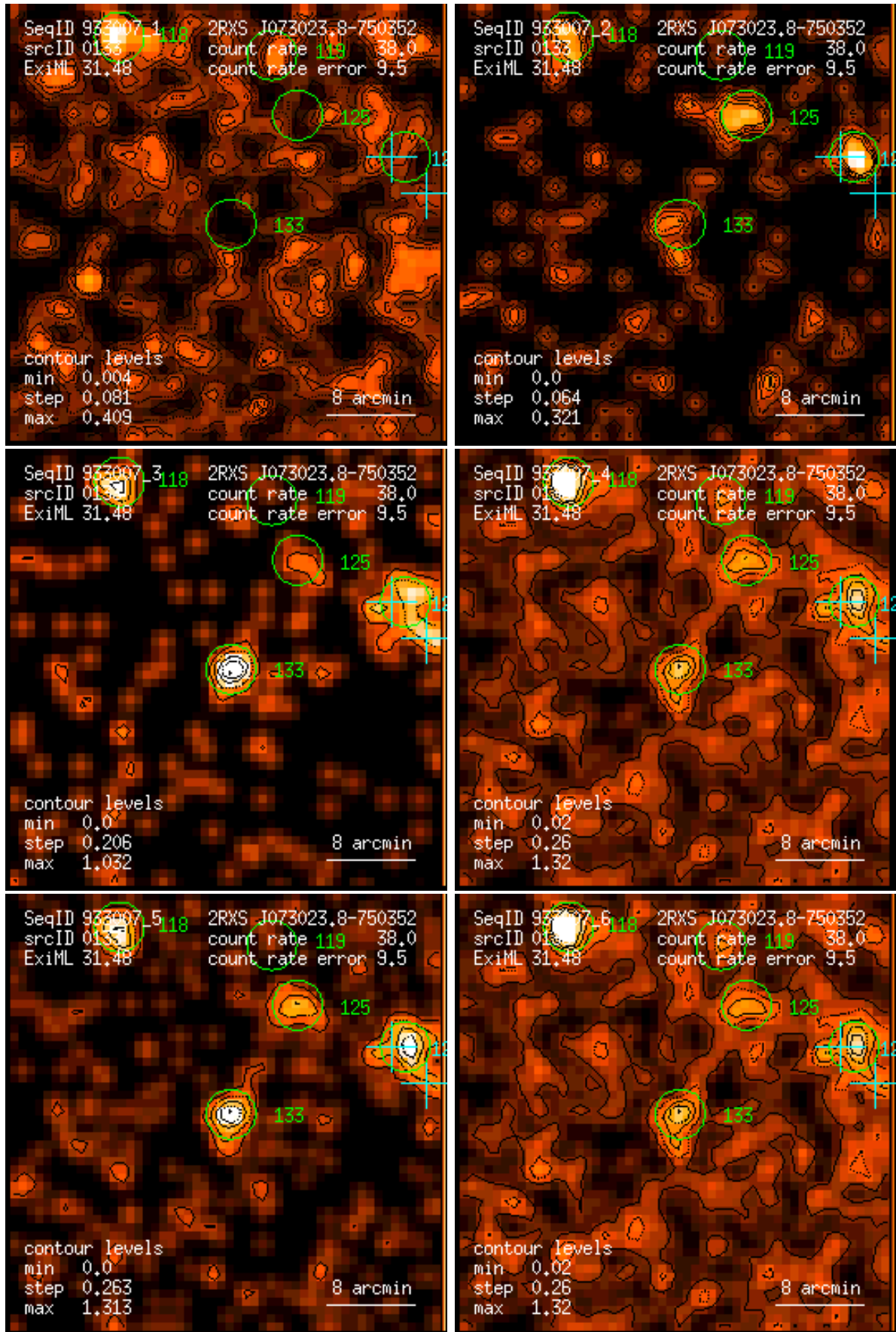
Figure 133: RASS 933007: detection 0133: band rate images, Gaussian filter: (1) PSPC channels 11 – 41, (2) 52 – 90, (3) 91 – 201, (4) 11 – 235, (5) 52 – 201, (6) 11 – 201. Broad band rates in counts/ks. Band rate contour levels in counts/ks/arcmin 2 .
