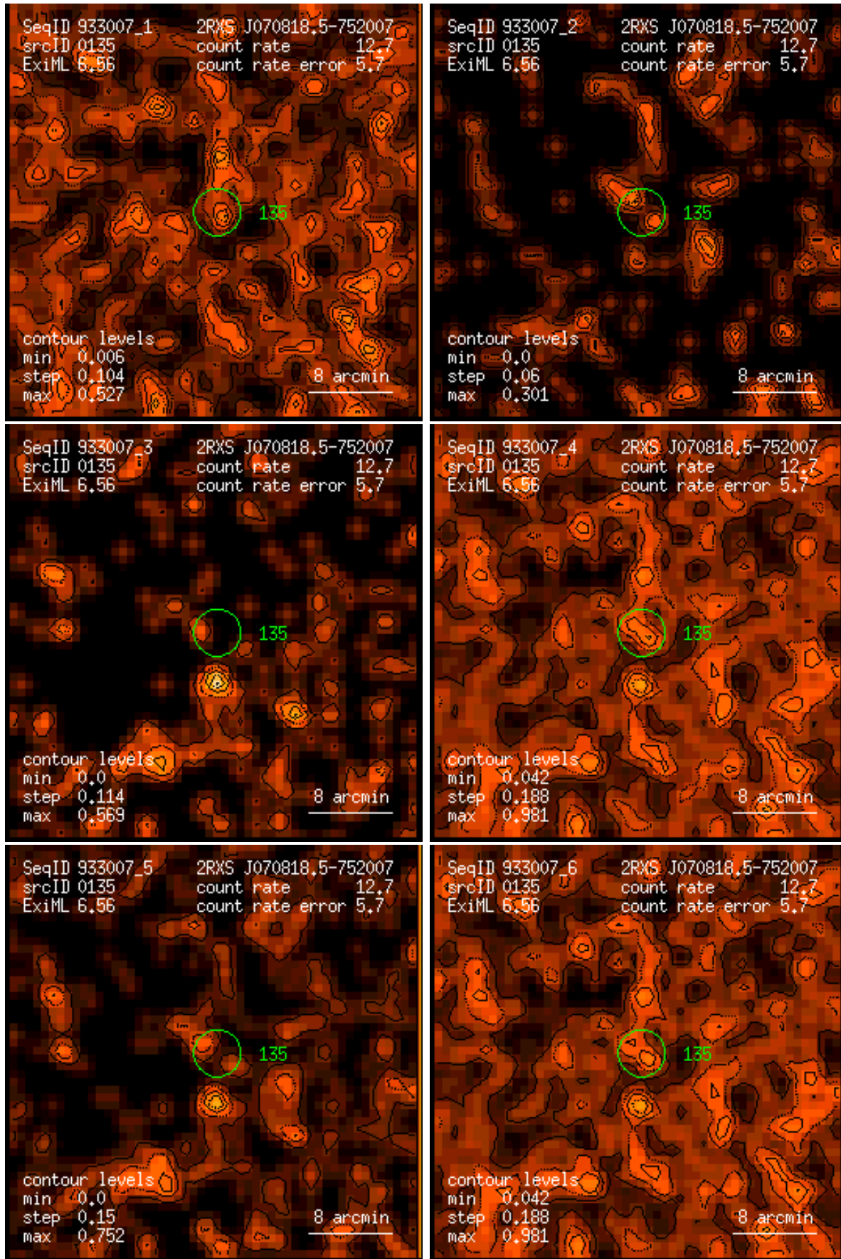
Figure 135: RASS 933007: detection 0135: band rate images, Gaussian filter: (1) PSPC channels 11 – 41, (2) 52 – 90, (3) 91 – 201, (4) 11 – 235, (5) 52 – 201, (6) 11 – 201. Broad band rates in counts/ks. Band rate contour levels in counts/ks/arcmin 2 .
