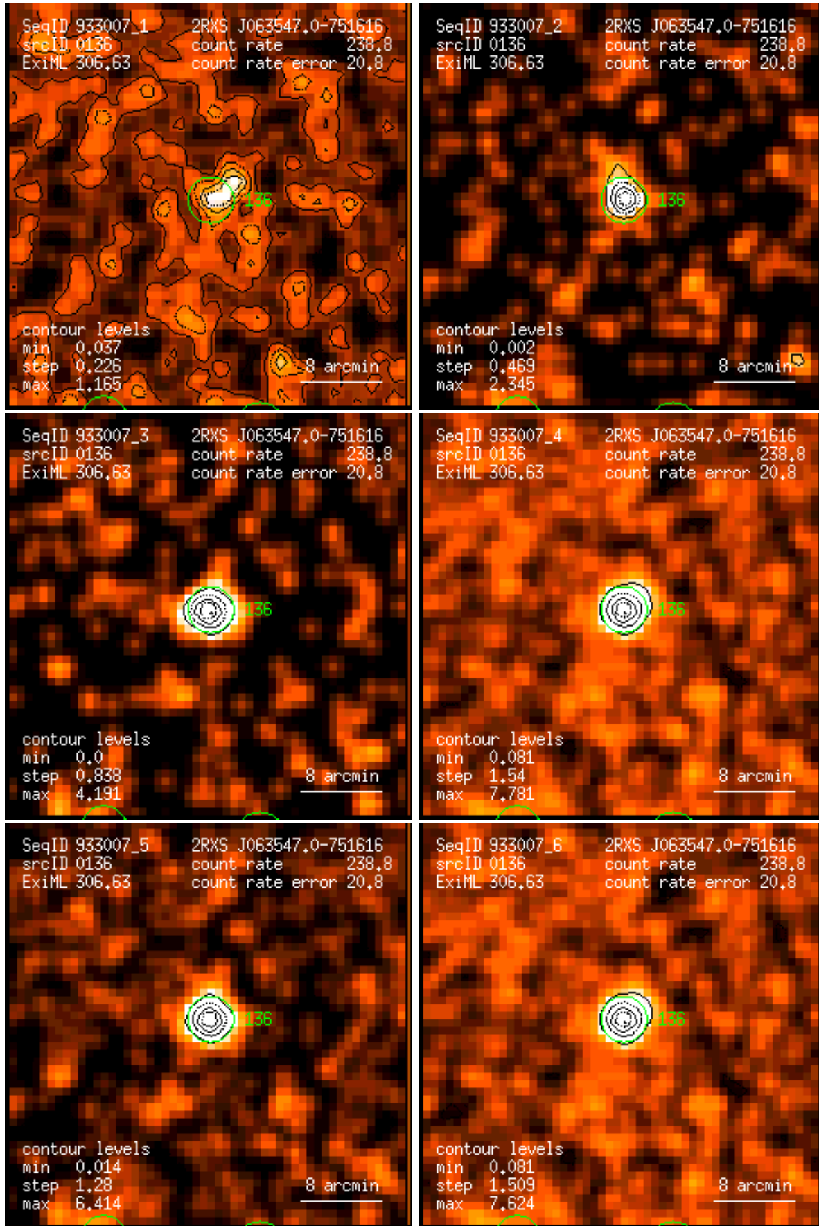
Figure 136: RASS 933007: detection 0136: band rate images, Gaussian filter: (1) PSPC channels 11 – 41, (2) 52 – 90, (3) 91 – 201, (4) 11 – 235, (5) 52 – 201, (6) 11 – 201. Broad band rates in counts/ks. Band rate contour levels in counts/ks/arcmin 2 .
