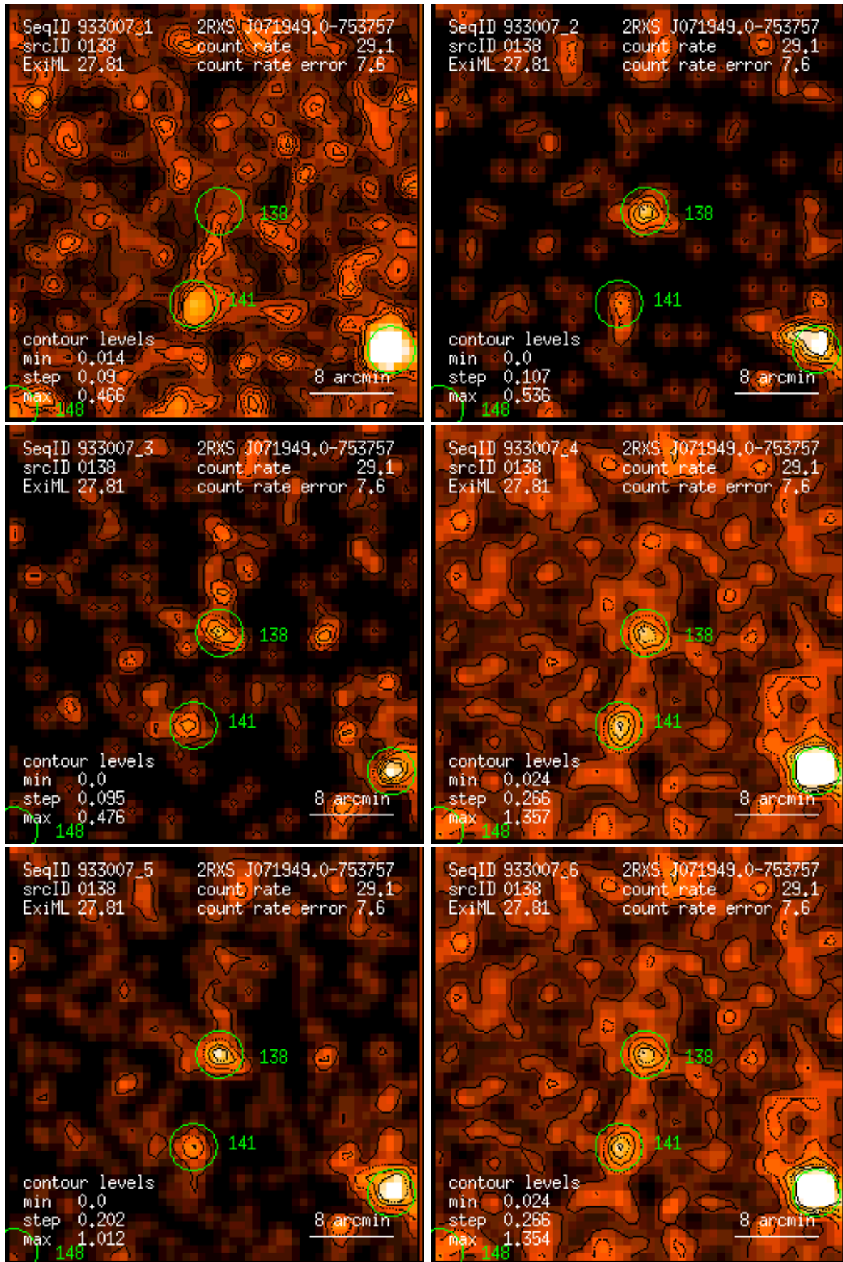
Figure 138: RASS 933007: detection 0138: band rate images, Gaussian filter: (1) PSPC channels 11 – 41, (2) 52 – 90, (3) 91 – 201, (4) 11 – 235, (5) 52 – 201, (6) 11 – 201. Broad band rates in counts/ks. Band rate contour levels in counts/ks/arcmin 2 .
