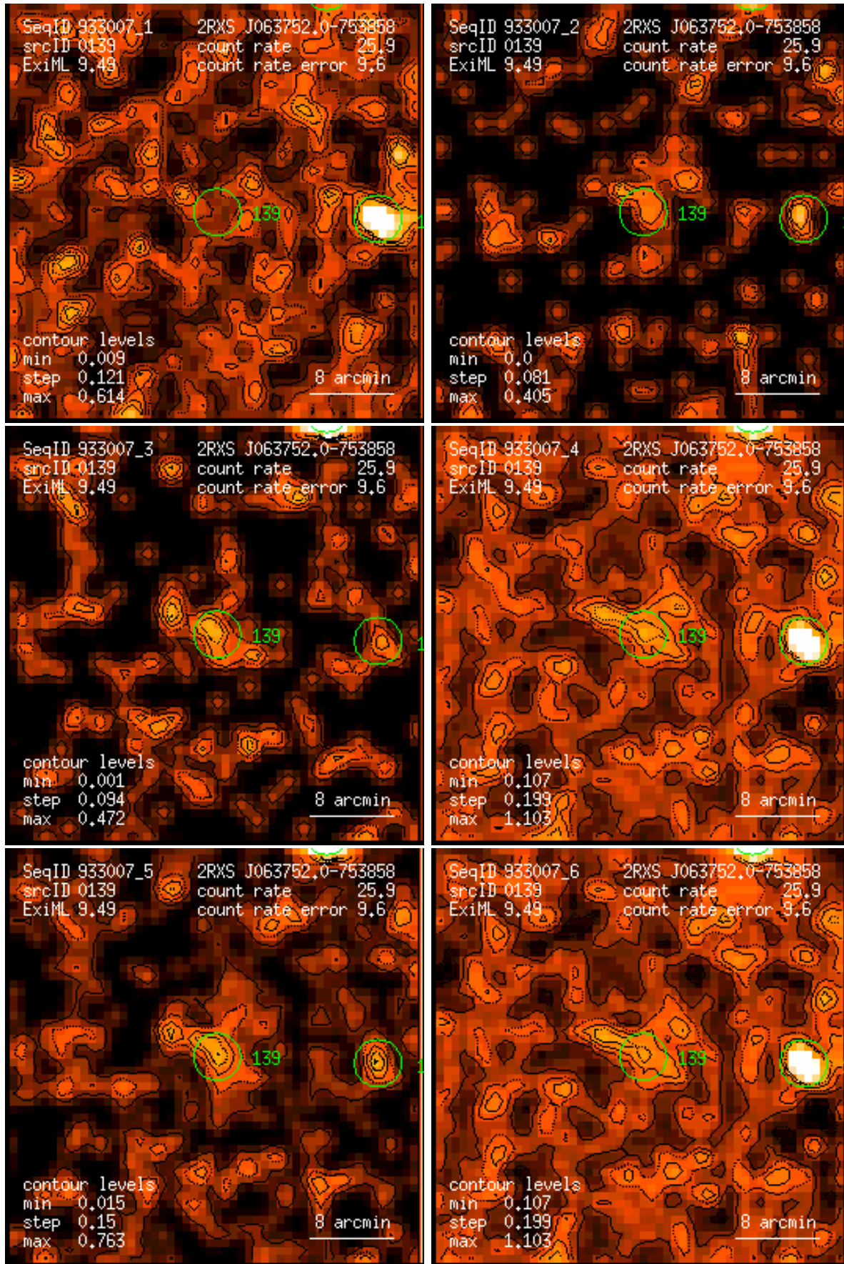
Figure 139: RASS 933007: detection 0139: band rate images, Gaussian filter: (1) PSPC channels 11 – 41, (2) 52 – 90, (3) 91 – 201, (4) 11 – 235, (5) 52 – 201, (6) 11 – 201. Broad band rates in counts/ks. Band rate contour levels in counts/ks/arcmin 2 .
