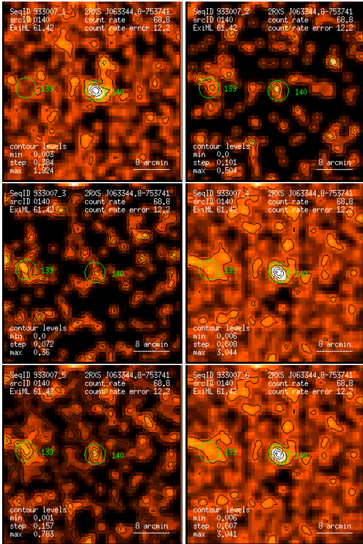
Figure 140: RASS 933007: detection 0140: band rate images, Gaussian filter: (1) PSPC channels 11 – 41, (2) 52 – 90, (3) 91 – 201, (4) 11 – 235, (5) 52 – 201, (6) 11 – 201. Broad band rates in counts/ks. Band rate contour levels in counts/ks/arcmin 2 .
