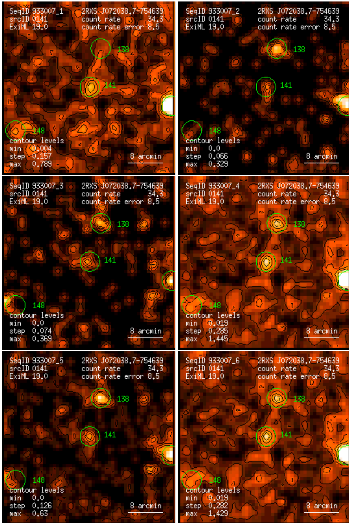
Figure 141: RASS 933007: detection 0141: band rate images, Gaussian filter: (1) PSPC channels 11 – 41, (2) 52 – 90, (3) 91 – 201, (4) 11 – 235, (5) 52 – 201, (6) 11 – 201. Broad band rates in counts/ks. Band rate contour levels in counts/ks/arcmin 2 .
