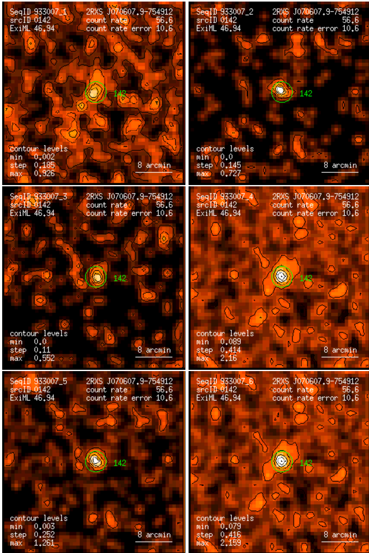
Figure 142: RASS 933007: detection 0142: band rate images, Gaussian filter: (1) PSPC channels 11 – 41, (2) 52 – 90, (3) 91 – 201, (4) 11 – 235, (5) 52 – 201, (6) 11 – 201. Broad band rates in counts/ks. Band rate contour levels in counts/ks/arcmin 2 .
