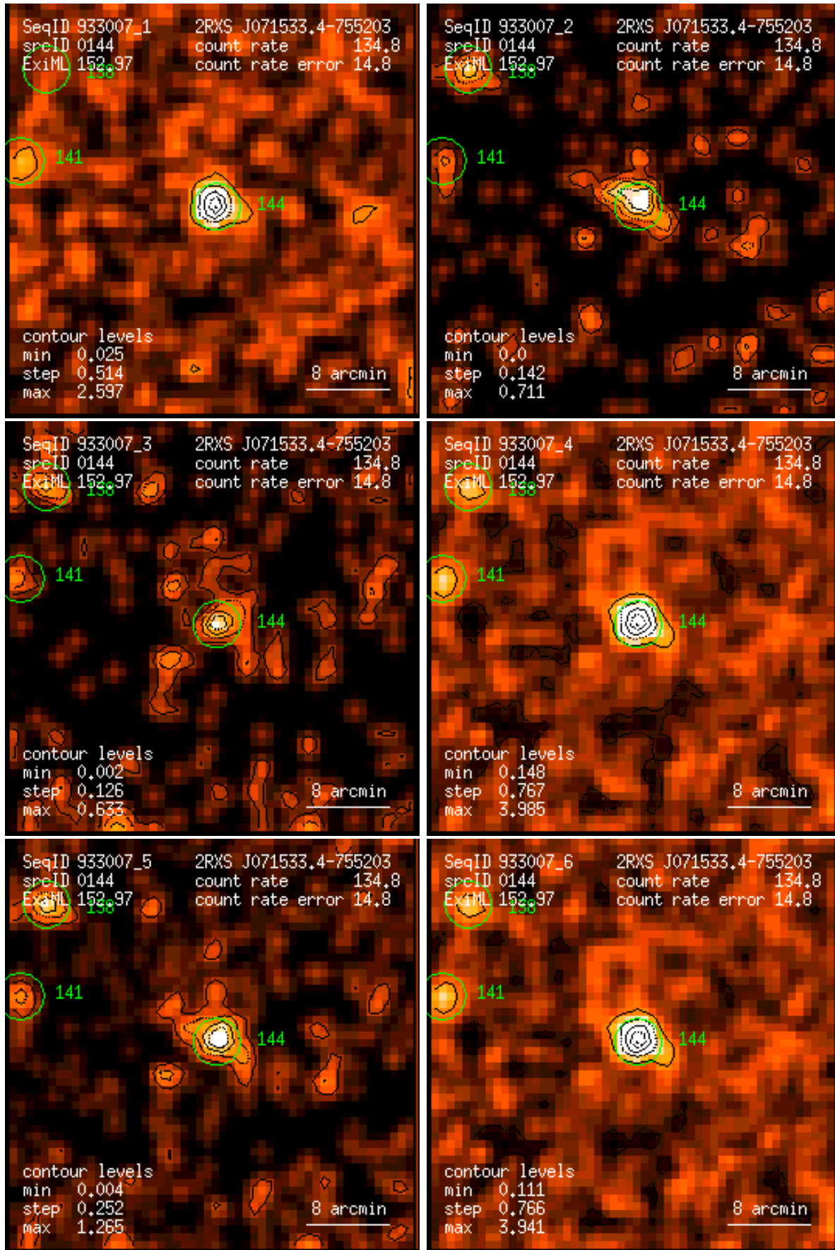
Figure 144: RASS 933007: detection 0144: band rate images, Gaussian filter: (1) PSPC channels 11 – 41, (2) 52 – 90, (3) 91 – 201, (4) 11 – 235, (5) 52 – 201, (6) 11 – 201. Broad band rates in counts/ks. Band rate contour levels in counts/ks/arcmin 2 .
