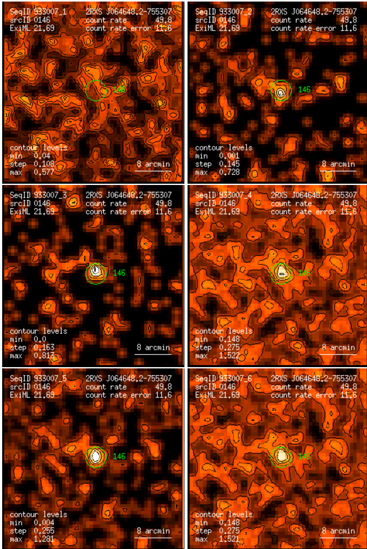
Figure 146: RASS 933007: detection 0146: band rate images, Gaussian filter: (1) PSPC channels 11 – 41, (2) 52 – 90, (3) 91 – 201, (4) 11 – 235, (5) 52 – 201, (6) 11 – 201. Broad band rates in counts/ks. Band rate contour levels in counts/ks/arcmin 2 .
