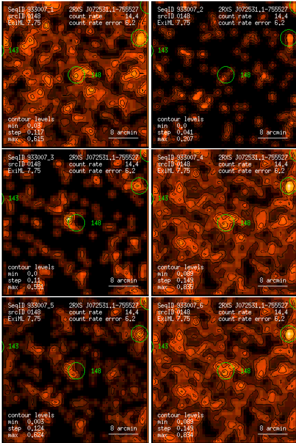
Figure 148: RASS 933007: detection 0148: band rate images, Gaussian filter: (1) PSPC channels 11 – 41, (2) 52 – 90, (3) 91 – 201, (4) 11 – 235, (5) 52 – 201, (6) 11 – 201. Broad band rates in counts/ks. Band rate contour levels in counts/ks/arcmin 2 .
