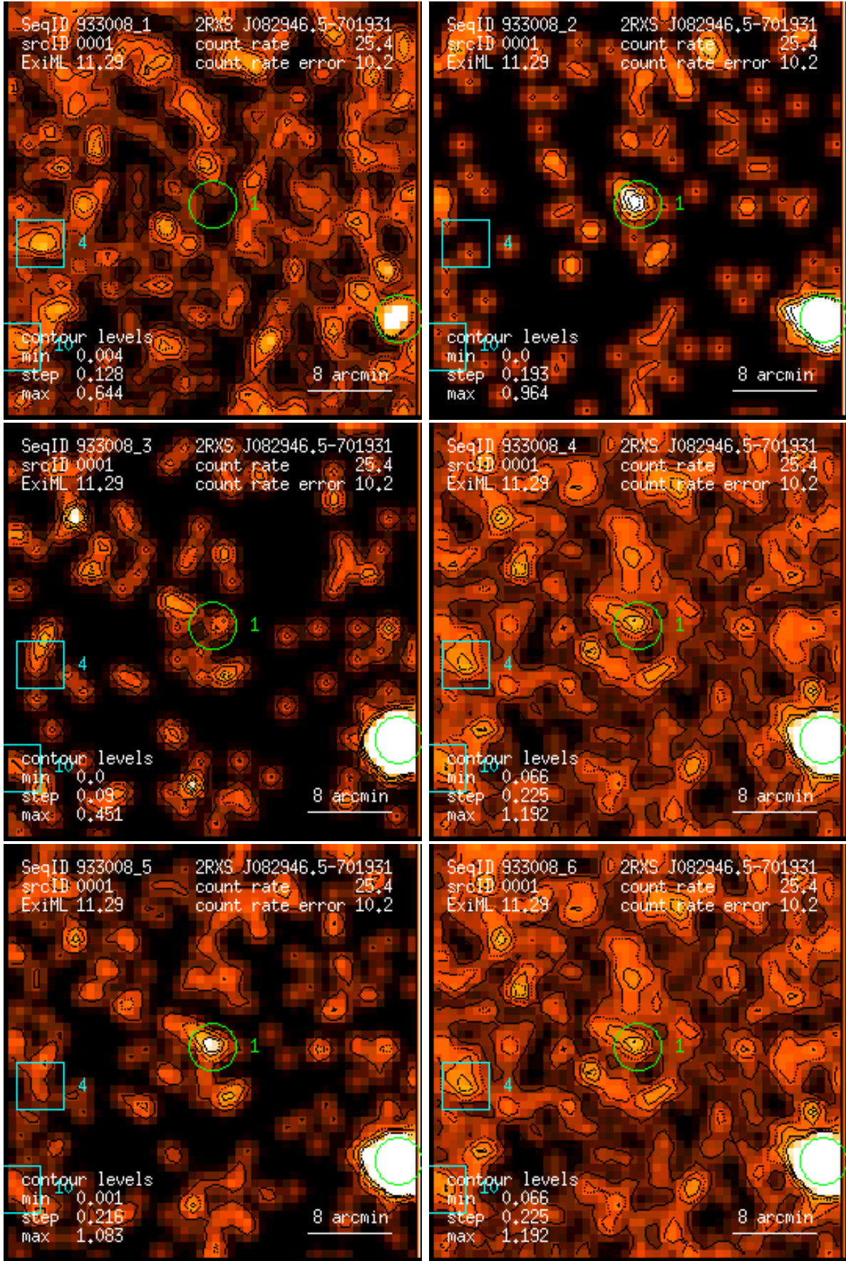
Figure 1: RASS 933008: detection 0001: band rate images, Gaussian filter: (1) PSPC channels 11 – 41, (2) 52 – 90, (3) 91 – 201, (4) 11 – 235, (5) 52 – 201, (6) 11 – 201. Broad band rates in counts/ks. Band rate contour levels in counts/ks/arcmin 2 .
