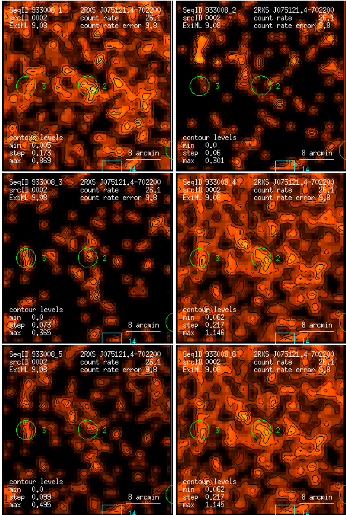
Figure 2: RASS 933008: detection 0002: band rate images, Gaussian filter: (1) PSPC channels 11 – 41, (2) 52 – 90, (3) 91 – 201, (4) 11 – 235, (5) 52 – 201, (6) 11 – 201. Broad band rates in counts/ks. Band rate contour levels in counts/ks/arcmin 2 .
