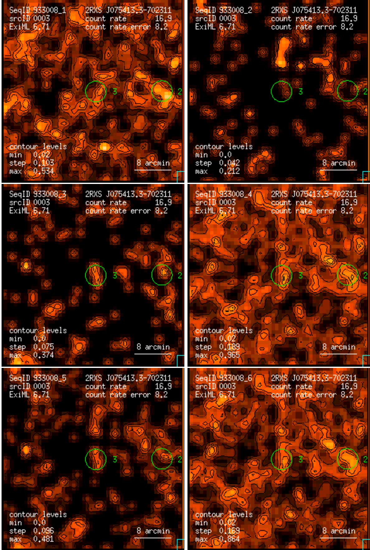
Figure 3: RASS 933008: detection 0003: band rate images, Gaussian filter: (1) PSPC channels 11 – 41, (2) 52 – 90, (3) 91 – 201, (4) 11 – 235, (5) 52 – 201, (6) 11 – 201. Broad band rates in counts/ks. Band rate contour levels in counts/ks/arcmin 2 .
