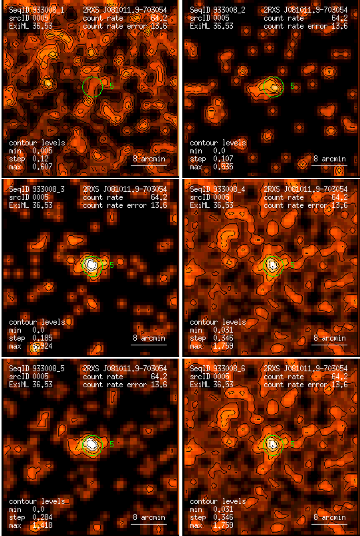
Figure 5: RASS 933008: detection 0005: band rate images, Gaussian filter: (1) PSPC channels 11 – 41, (2) 52 – 90, (3) 91 – 201, (4) 11 – 235, (5) 52 – 201, (6) 11 – 201. Broad band rates in counts/ks. Band rate contour levels in counts/ks/arcmin 2 .
