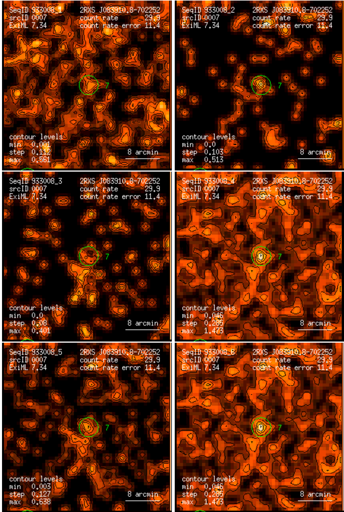
Figure 7: RASS 933008: detection 0007: band rate images, Gaussian filter: (1) PSPC channels 11 – 41, (2) 52 – 90, (3) 91 – 201, (4) 11 – 235, (5) 52 – 201, (6) 11 – 201. Broad band rates in counts/ks. Band rate contour levels in counts/ks/arcmin 2 .
