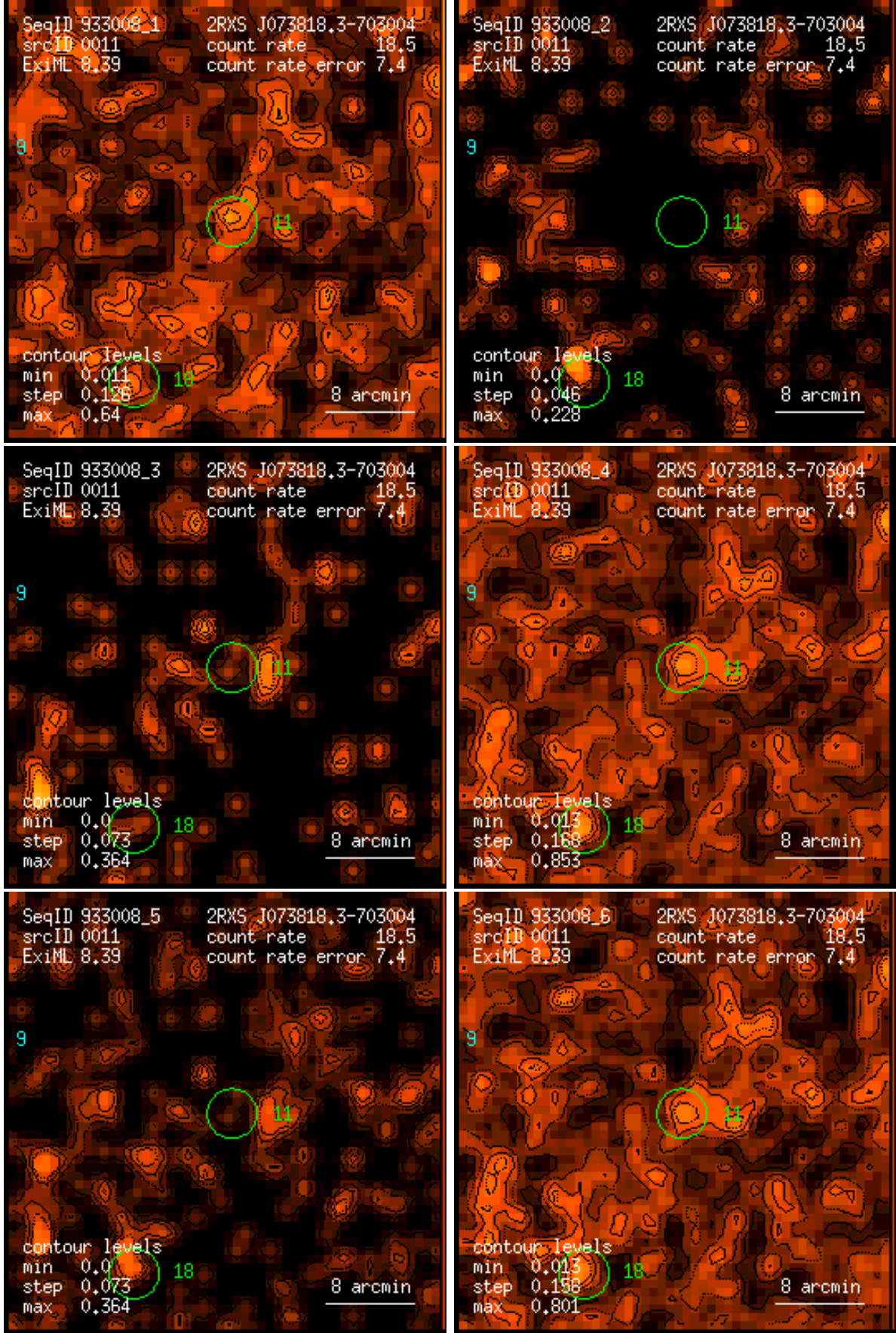
Figure 11: RASS 933008: detection 0011: band rate images, Gaussian filter: (1) PSPC channels 11 – 41, (2) 52 – 90, (3) 91 – 201, (4) 11 – 235, (5) 52 – 201, (6) 11 – 201. Broad band rates in counts/ks. Band rate contour levels in counts/ks/arcmin 2 .
