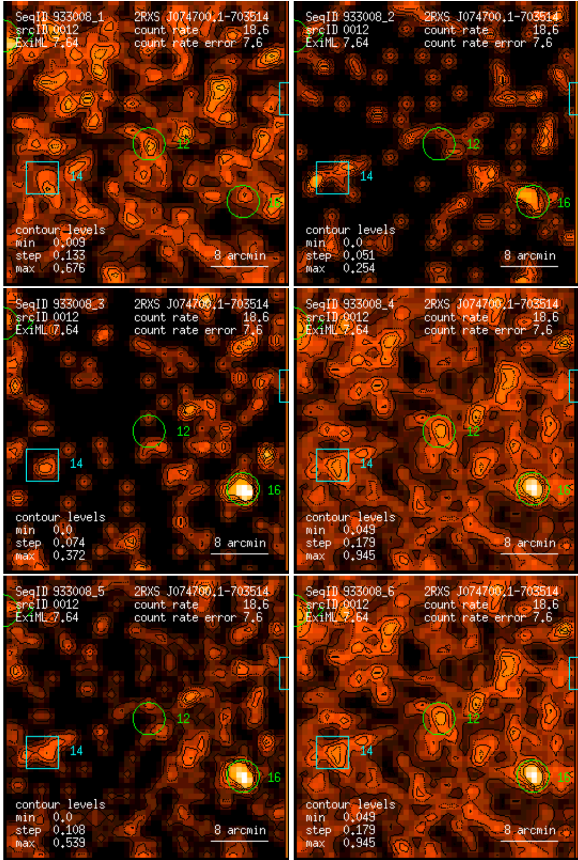
Figure 12: RASS 933008: detection 0012: band rate images, Gaussian filter: (1) PSPC channels 11 – 41, (2) 52 – 90, (3) 91 – 201, (4) 11 – 235, (5) 52 – 201, (6) 11 – 201. Broad band rates in counts/ks. Band rate contour levels in counts/ks/arcmin 2 .
