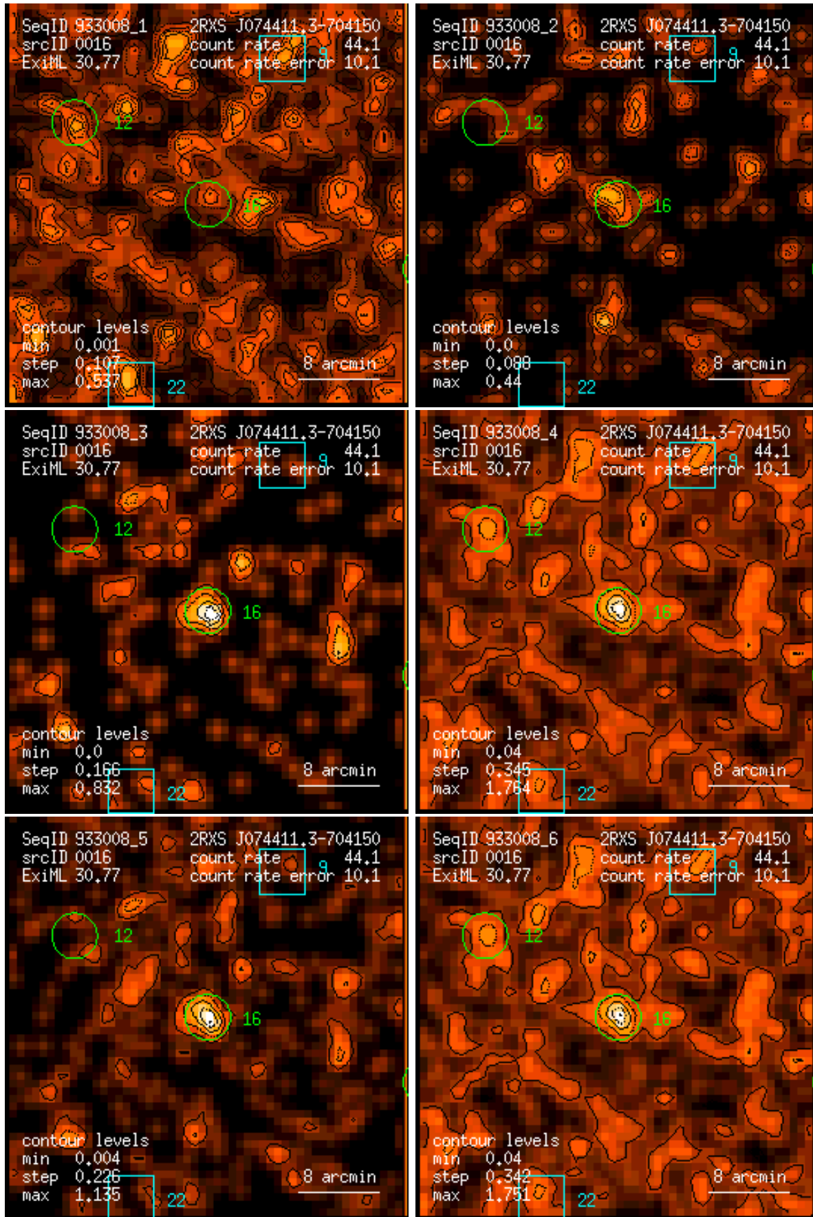
Figure 16: RASS 933008: detection 0016: band rate images, Gaussian filter: (1) PSPC channels 11 – 41, (2) 52 – 90, (3) 91 – 201, (4) 11 – 235, (5) 52 – 201, (6) 11 – 201. Broad band rates in counts/ks. Band rate contour levels in counts/ks/arcmin 2 .
