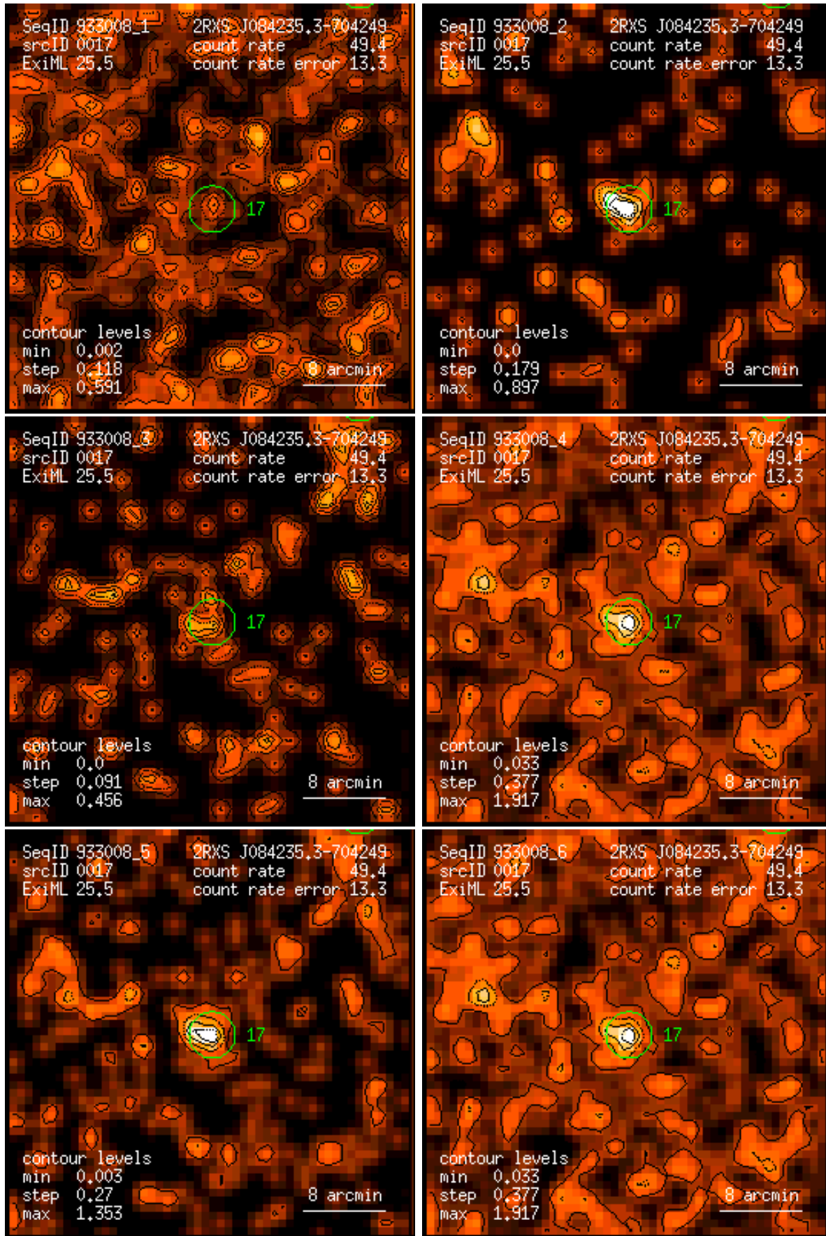
Figure 17: RASS 933008: detection 0017: band rate images, Gaussian filter: (1) PSPC channels 11 – 41, (2) 52 – 90, (3) 91 – 201, (4) 11 – 235, (5) 52 – 201, (6) 11 – 201. Broad band rates in counts/ks. Band rate contour levels in counts/ks/arcmin 2 .
