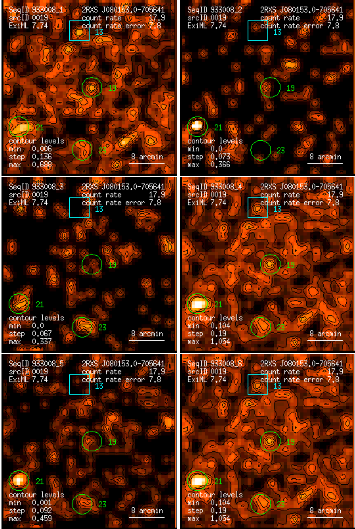
Figure 19: RASS 933008: detection 0019: band rate images, Gaussian filter: (1) PSPC channels 11 – 41, (2) 52 – 90, (3) 91 – 201, (4) 11 – 235, (5) 52 – 201, (6) 11 – 201. Broad band rates in counts/ks. Band rate contour levels in counts/ks/arcmin 2 .
