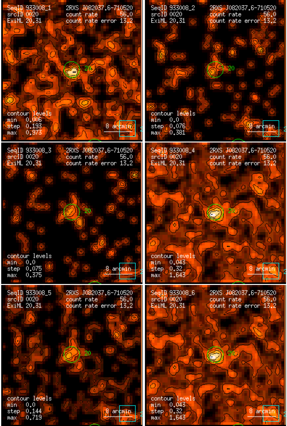
Figure 20: RASS 933008: detection 0020: band rate images, Gaussian filter: (1) PSPC channels 11 – 41, (2) 52 – 90, (3) 91 – 201, (4) 11 – 235, (5) 52 – 201, (6) 11 – 201. Broad band rates in counts/ks. Band rate contour levels in counts/ks/arcmin 2 .
