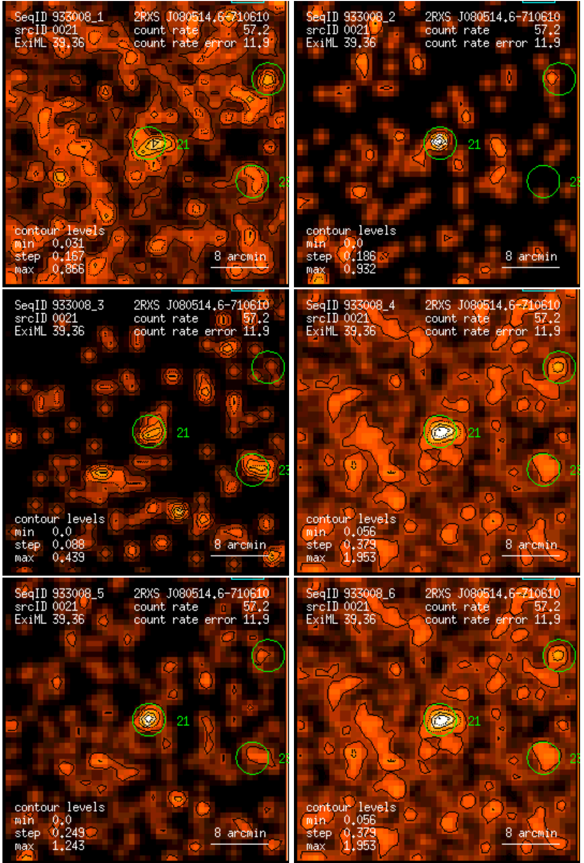
Figure 21: RASS 933008: detection 0021: band rate images, Gaussian filter: (1) PSPC channels 11 – 41, (2) 52 – 90, (3) 91 – 201, (4) 11 – 235, (5) 52 – 201, (6) 11 – 201. Broad band rates in counts/ks. Band rate contour levels in counts/ks/arcmin 2 .
