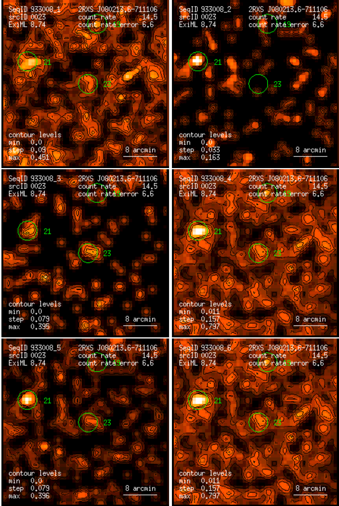
Figure 23: RASS 933008: detection 0023: band rate images, Gaussian filter: (1) PSPC channels 11 – 41, (2) 52 – 90, (3) 91 – 201, (4) 11 – 235, (5) 52 – 201, (6) 11 – 201. Broad band rates in counts/ks. Band rate contour levels in counts/ks/arcmin 2 .
