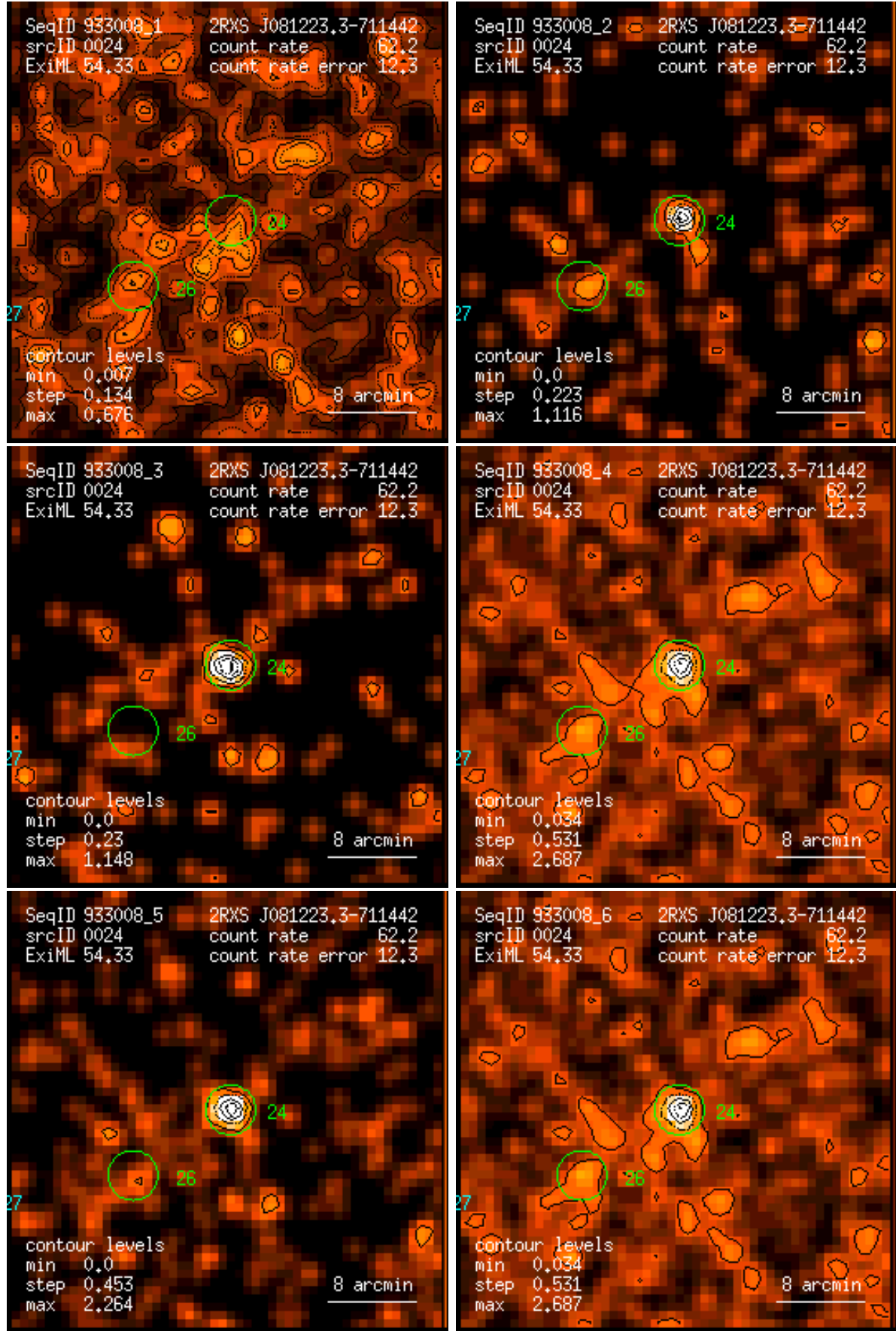
Figure 24: RASS 933008: detection 0024: band rate images, Gaussian filter: (1) PSPC channels 11 – 41, (2) 52 – 90, (3) 91 – 201, (4) 11 – 235, (5) 52 – 201, (6) 11 – 201. Broad band rates in counts/ks. Band rate contour levels in counts/ks/arcmin 2 .
