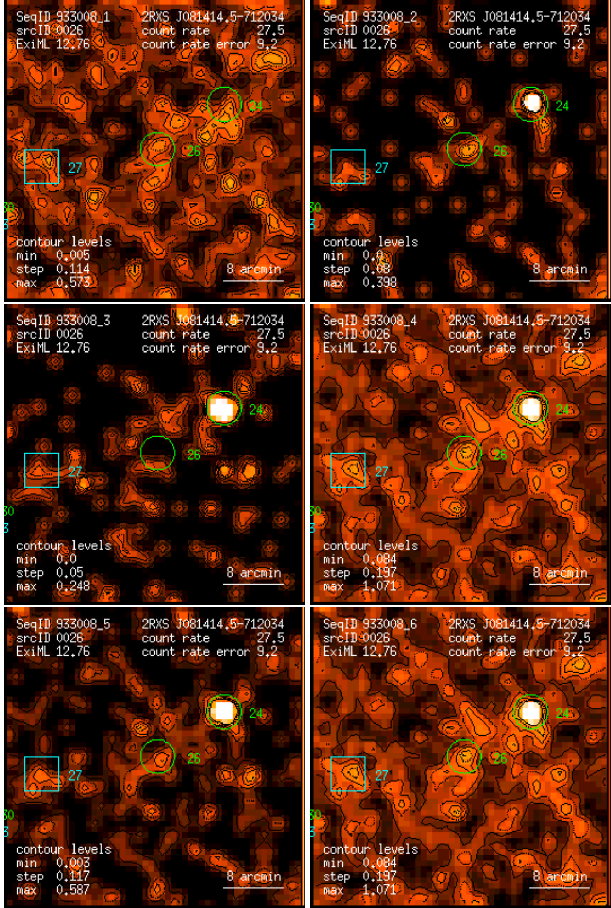
Figure 26: RASS 933008: detection 0026: band rate images, Gaussian filter: (1) PSPC channels 11 – 41, (2) 52 – 90, (3) 91 – 201, (4) 11 – 235, (5) 52 – 201, (6) 11 – 201. Broad band rates in counts/ks. Band rate contour levels in counts/ks/arcmin 2 .
