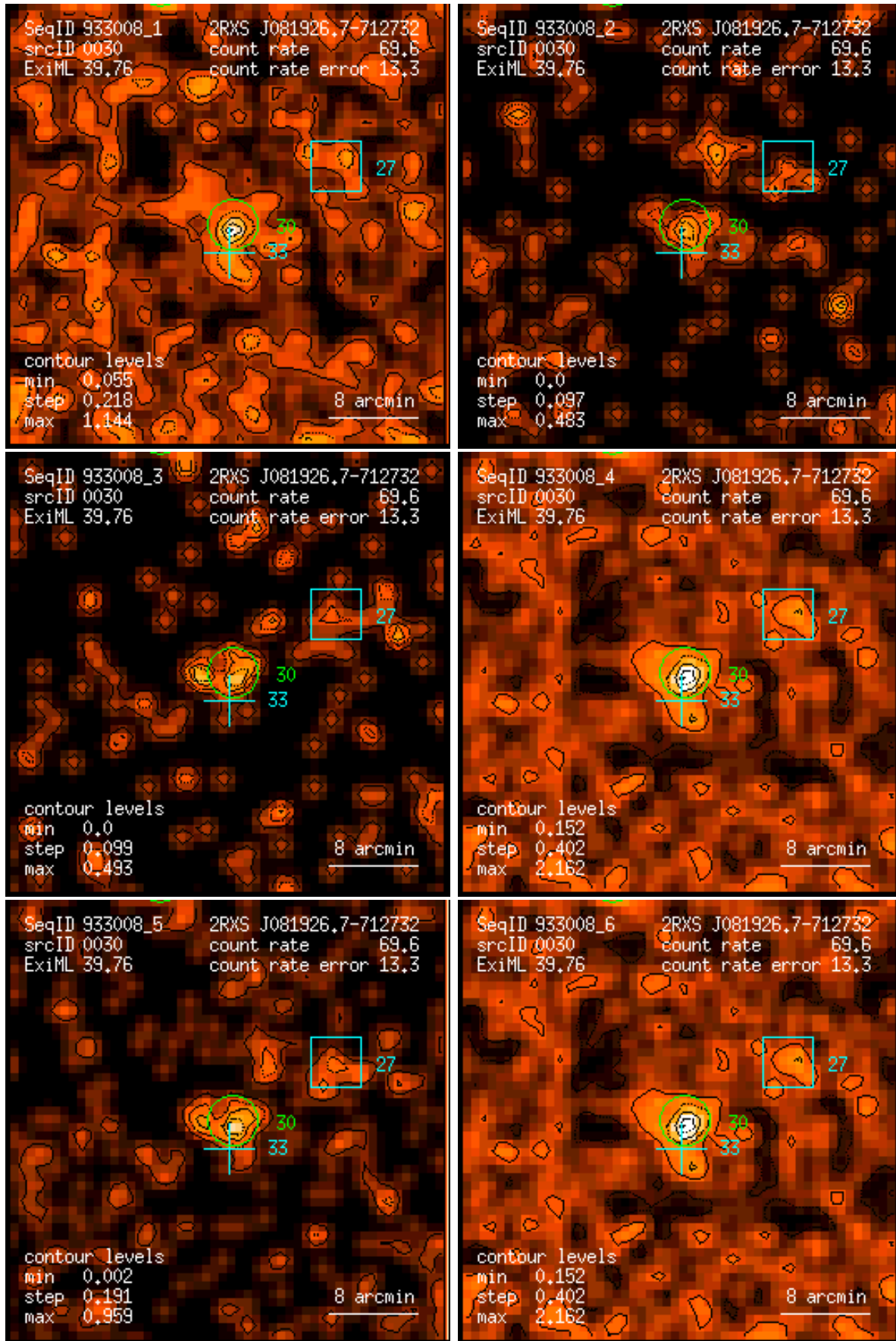
Figure 30: RASS 933008: detection 0030: band rate images, Gaussian filter: (1) PSPC channels 11 – 41, (2) 52 – 90, (3) 91 – 201, (4) 11 – 235, (5) 52 – 201, (6) 11 – 201. Broad band rates in counts/ks. Band rate contour levels in counts/ks/arcmin 2 .
