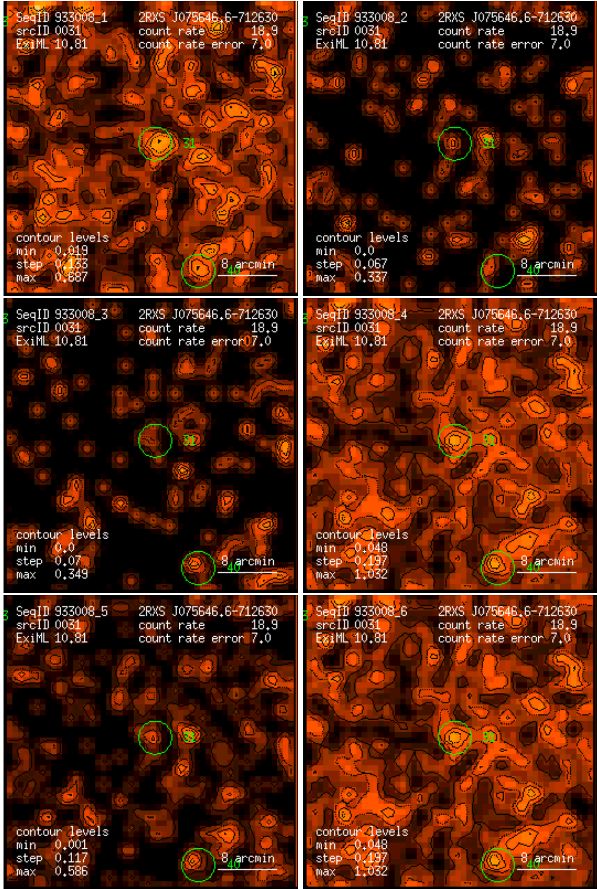
Figure 31: RASS 933008: detection 0031: band rate images, Gaussian filter: (1) PSPC channels 11 – 41, (2) 52 – 90, (3) 91 – 201, (4) 11 – 235, (5) 52 – 201, (6) 11 – 201. Broad band rates in counts/ks. Band rate contour levels in counts/ks/arcmin 2 .
