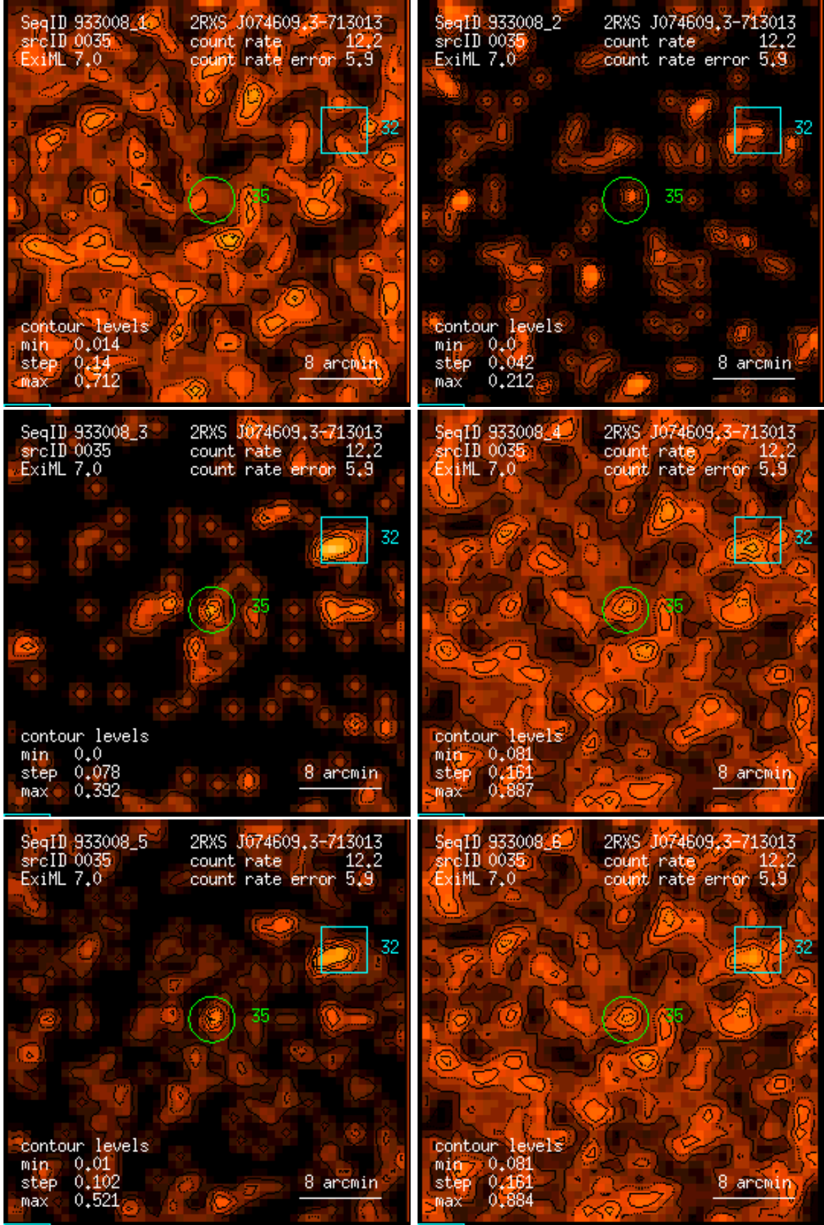
Figure 35: RASS 933008: detection 0035: band rate images, Gaussian filter: (1) PSPC channels 11 – 41, (2) 52 – 90, (3) 91 – 201, (4) 11 – 235, (5) 52 – 201, (6) 11 – 201. Broad band rates in counts/ks. Band rate contour levels in counts/ks/arcmin 2 .
