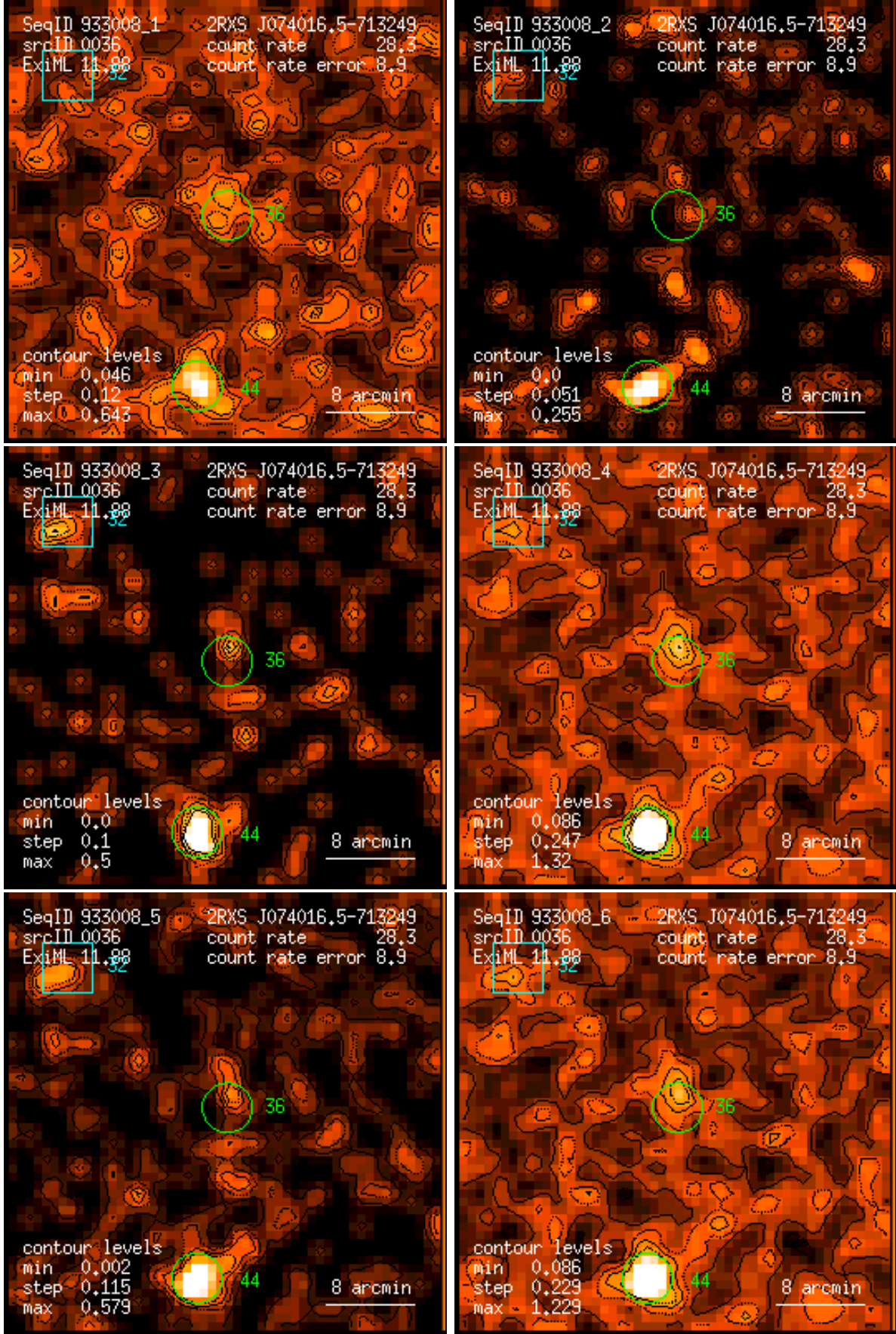
Figure 36: RASS 933008: detection 0036: band rate images, Gaussian filter: (1) PSPC channels 11 – 41, (2) 52 – 90, (3) 91 – 201, (4) 11 – 235, (5) 52 – 201, (6) 11 – 201. Broad band rates in counts/ks. Band rate contour levels in counts/ks/arcmin 2 .
