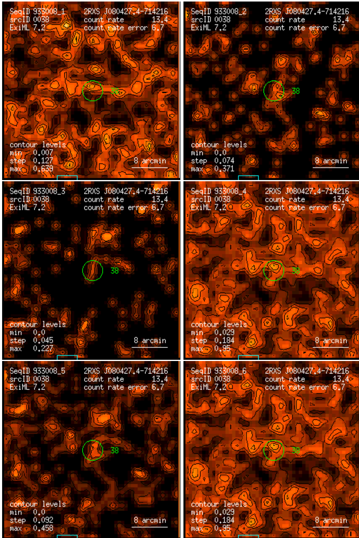
Figure 38: RASS 933008: detection 0038: band rate images, Gaussian filter: (1) PSPC channels 11 – 41, (2) 52 – 90, (3) 91 – 201, (4) 11 – 235, (5) 52 – 201, (6) 11 – 201. Broad band rates in counts/ks. Band rate contour levels in counts/ks/arcmin 2 .
