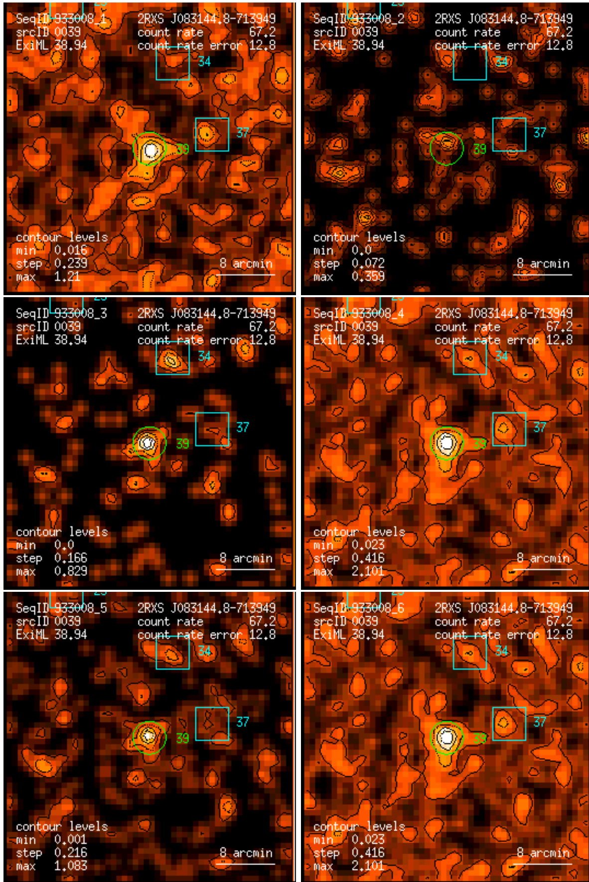
Figure 39: RASS 933008: detection 0039: band rate images, Gaussian filter: (1) PSPC channels 11 – 41, (2) 52 – 90, (3) 91 – 201, (4) 11 – 235, (5) 52 – 201, (6) 11 – 201. Broad band rates in counts/ks. Band rate contour levels in counts/ks/arcmin 2 .
