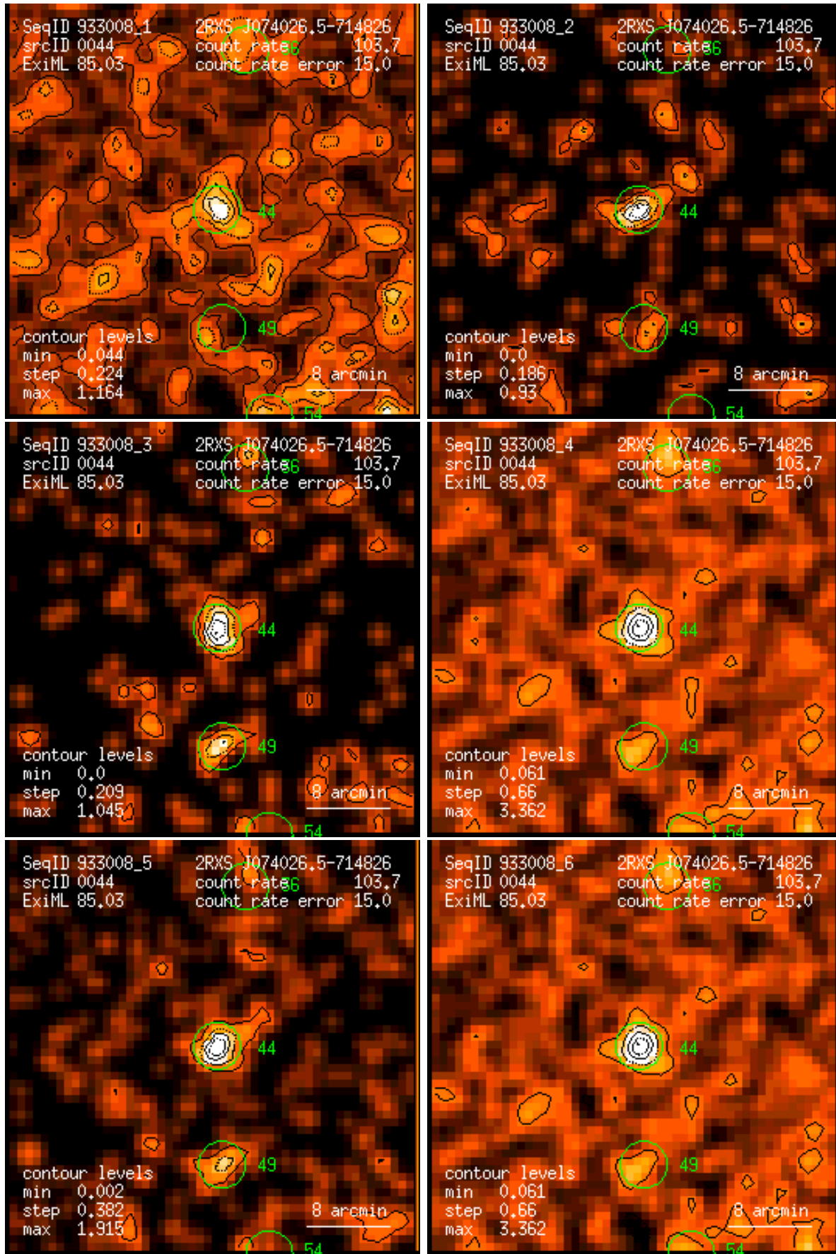
Figure 44: RASS 933008: detection 0044: band rate images, Gaussian filter: (1) PSPC channels 11 – 41, (2) 52 – 90, (3) 91 – 201, (4) 11 – 235, (5) 52 – 201, (6) 11 – 201. Broad band rates in counts/ks. Band rate contour levels in counts/ks/arcmin 2 .
