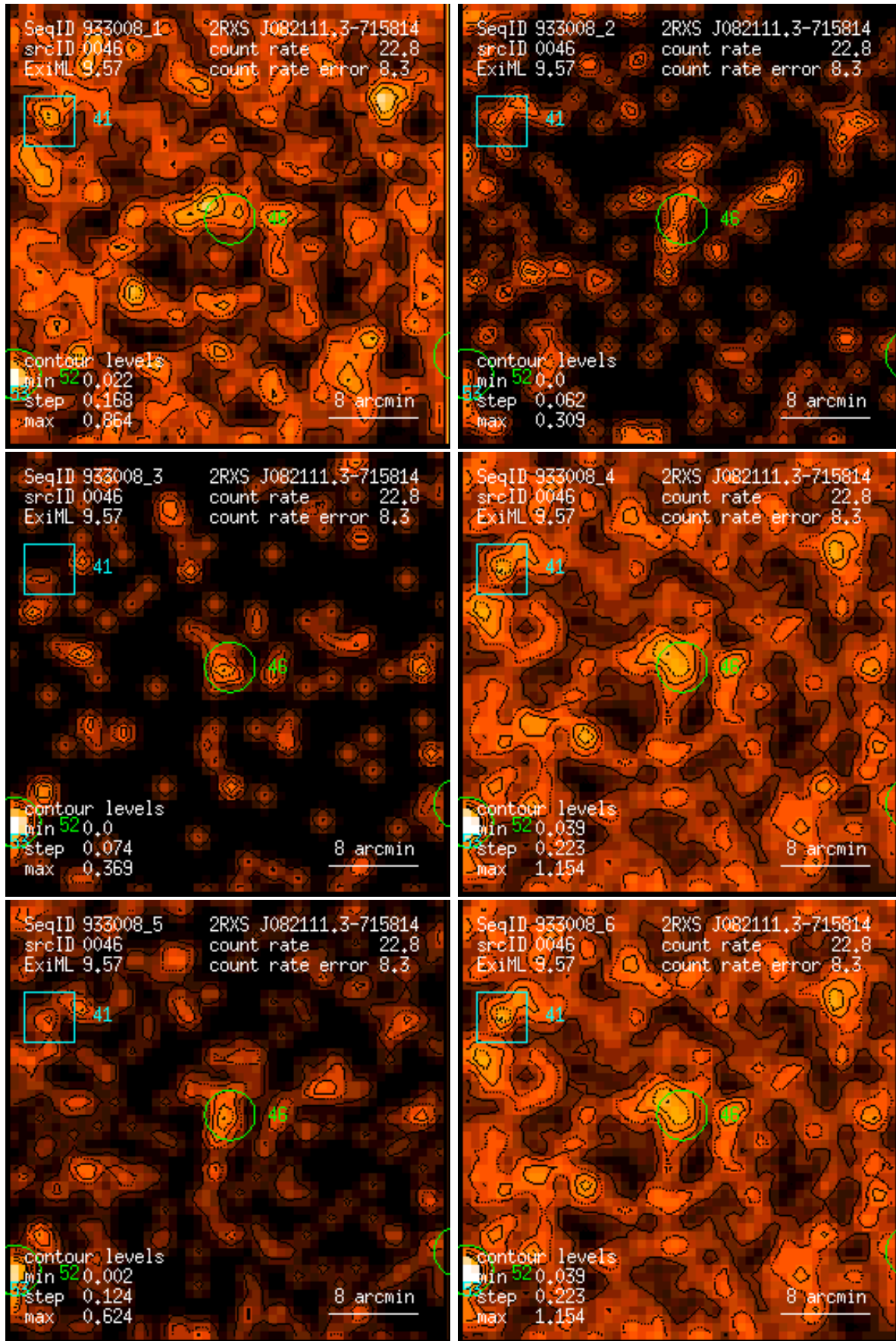
Figure 46: RASS 933008: detection 0046: band rate images, Gaussian filter: (1) PSPC channels 11 – 41, (2) 52 – 90, (3) 91 – 201, (4) 11 – 235, (5) 52 – 201, (6) 11 – 201. Broad band rates in counts/ks. Band rate contour levels in counts/ks/arcmin 2 .
