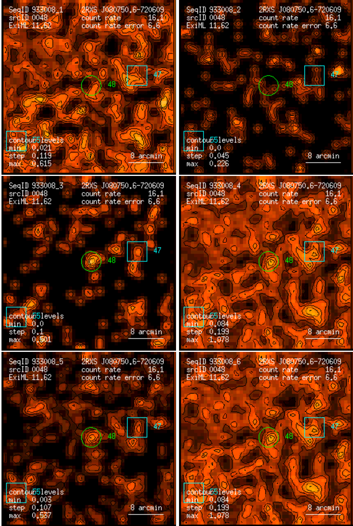
Figure 48: RASS 933008: detection 0048: band rate images, Gaussian filter: (1) PSPC channels 11 – 41, (2) 52 – 90, (3) 91 – 201, (4) 11 – 235, (5) 52 – 201, (6) 11 – 201. Broad band rates in counts/ks. Band rate contour levels in counts/ks/arcmin 2 .
