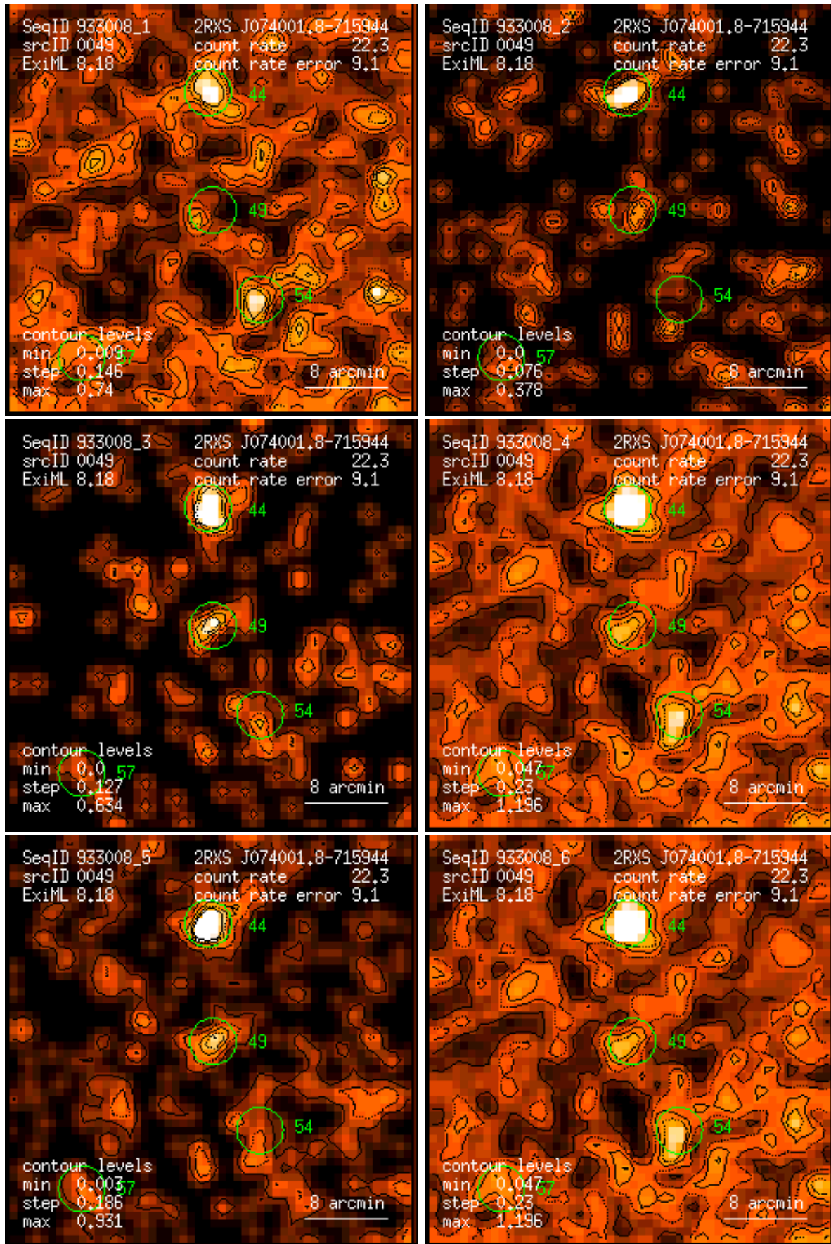
Figure 49: RASS 933008: detection 0049: band rate images, Gaussian filter: (1) PSPC channels 11 – 41, (2) 52 – 90, (3) 91 – 201, (4) 11 – 235, (5) 52 – 201, (6) 11 – 201. Broad band rates in counts/ks. Band rate contour levels in counts/ks/arcmin 2 .
