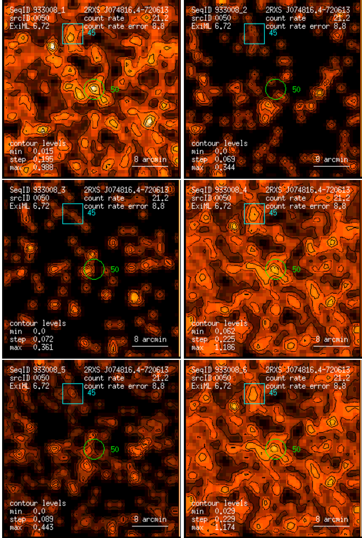
Figure 50: RASS 933008: detection 0050: band rate images, Gaussian filter: (1) PSPC channels 11 – 41, (2) 52 – 90, (3) 91 – 201, (4) 11 – 235, (5) 52 – 201, (6) 11 – 201. Broad band rates in counts/ks. Band rate contour levels in counts/ks/arcmin 2 .
