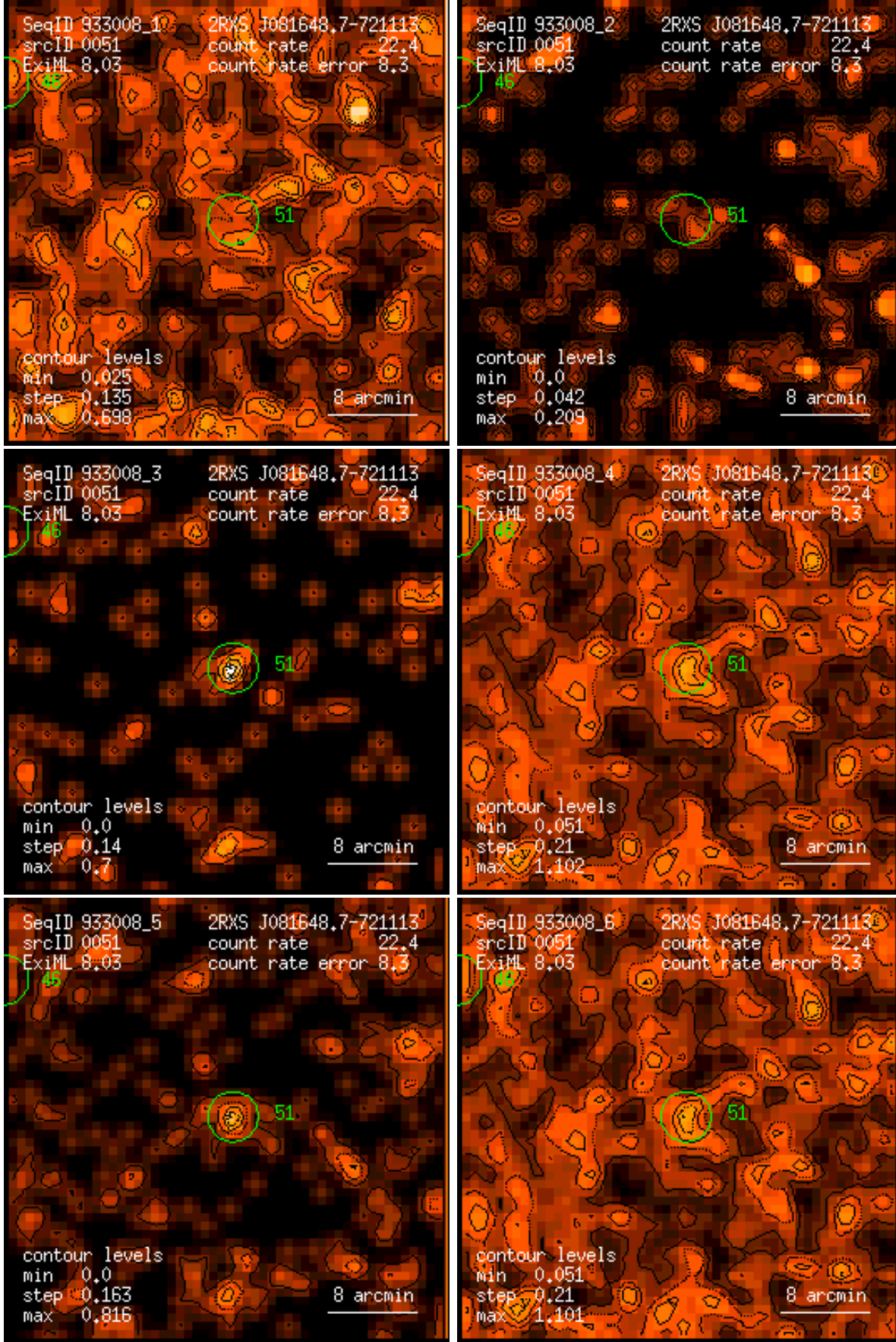
Figure 51: RASS 933008: detection 0051: band rate images, Gaussian filter: (1) PSPC channels 11 – 41, (2) 52 – 90, (3) 91 – 201, (4) 11 – 235, (5) 52 – 201, (6) 11 – 201. Broad band rates in counts/ks. Band rate contour levels in counts/ks/arcmin 2 .
