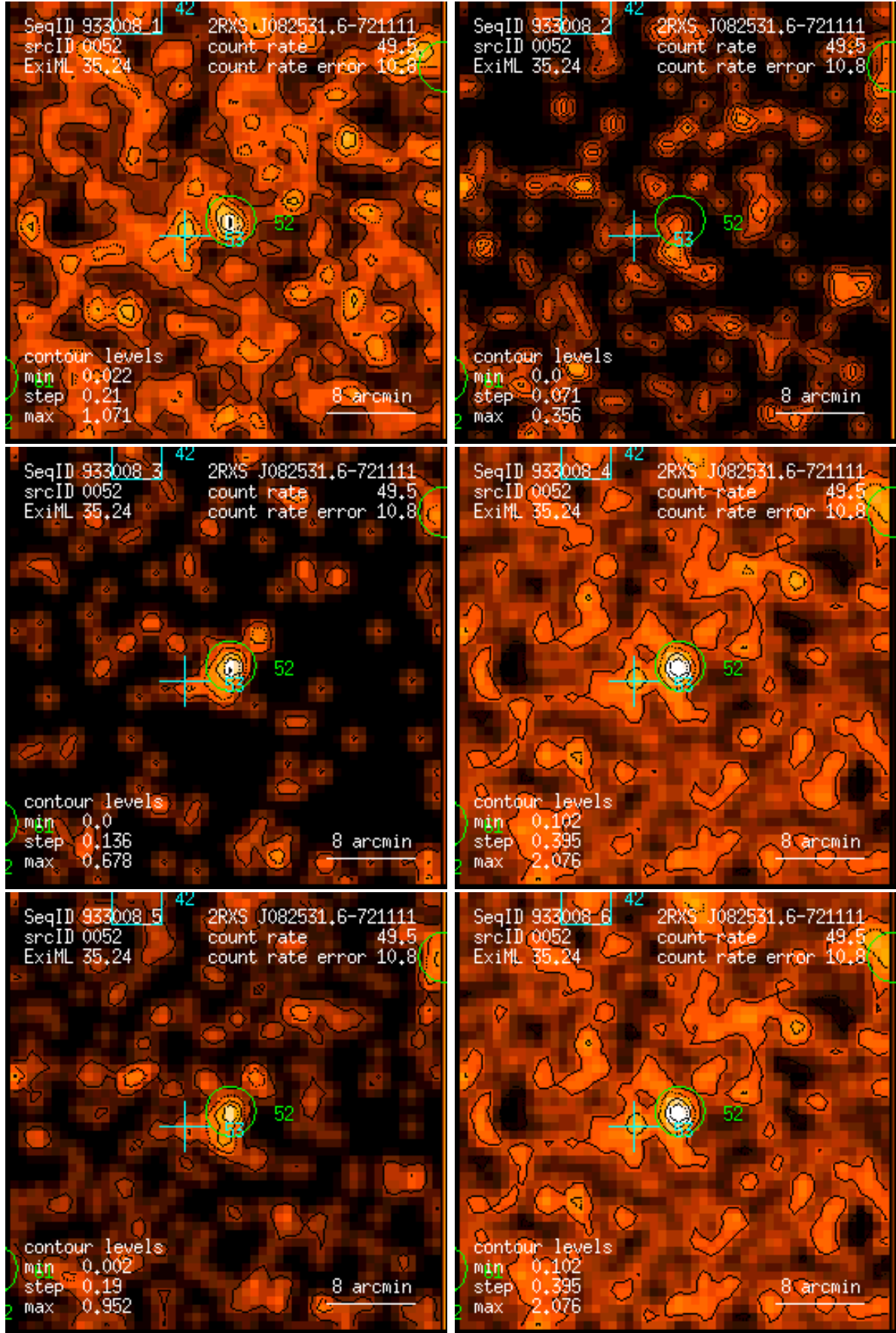
Figure 52: RASS 933008: detection 0052: band rate images, Gaussian filter: (1) PSPC channels 11 – 41, (2) 52 – 90, (3) 91 – 201, (4) 11 – 235, (5) 52 – 201, (6) 11 – 201. Broad band rates in counts/ks. Band rate contour levels in counts/ks/arcmin 2 .
