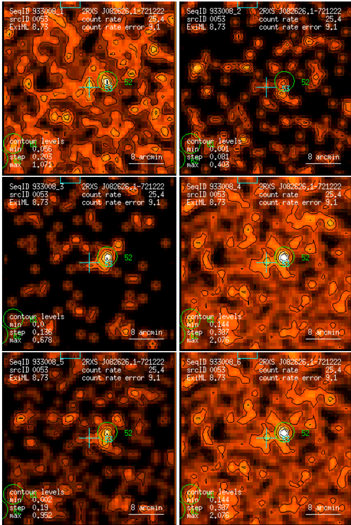
Figure 53: RASS 933008: detection 0053: band rate images, Gaussian filter: (1) PSPC channels 11 – 41, (2) 52 – 90, (3) 91 – 201, (4) 11 – 235, (5) 52 – 201, (6) 11 – 201. Broad band rates in counts/ks. Band rate contour levels in counts/ks/arcmin 2 .
