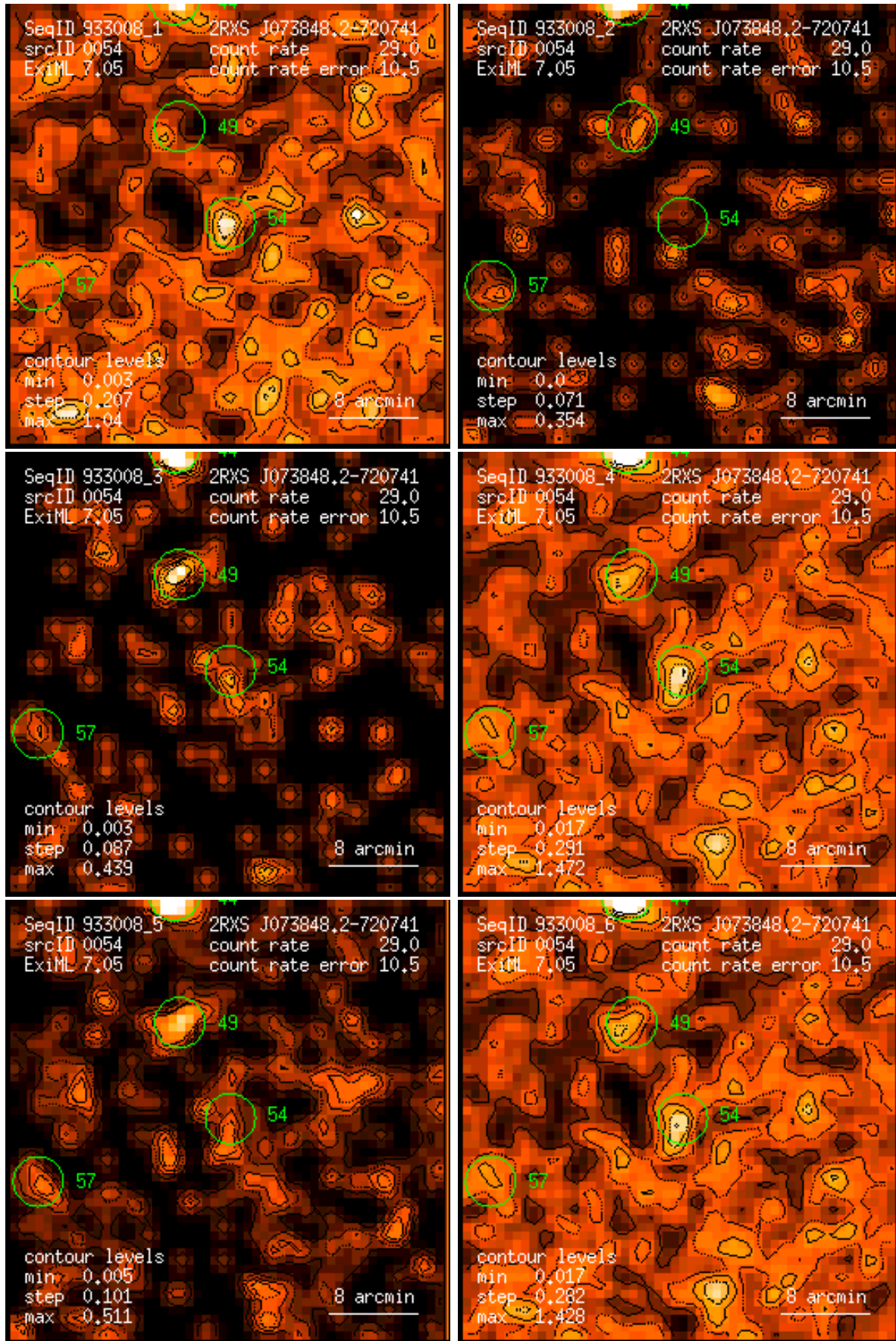
Figure 54: RASS 933008: detection 0054: band rate images, Gaussian filter: (1) PSPC channels 11 – 41, (2) 52 – 90, (3) 91 – 201, (4) 11 – 235, (5) 52 – 201, (6) 11 – 201. Broad band rates in counts/ks. Band rate contour levels in counts/ks/arcmin 2 .
