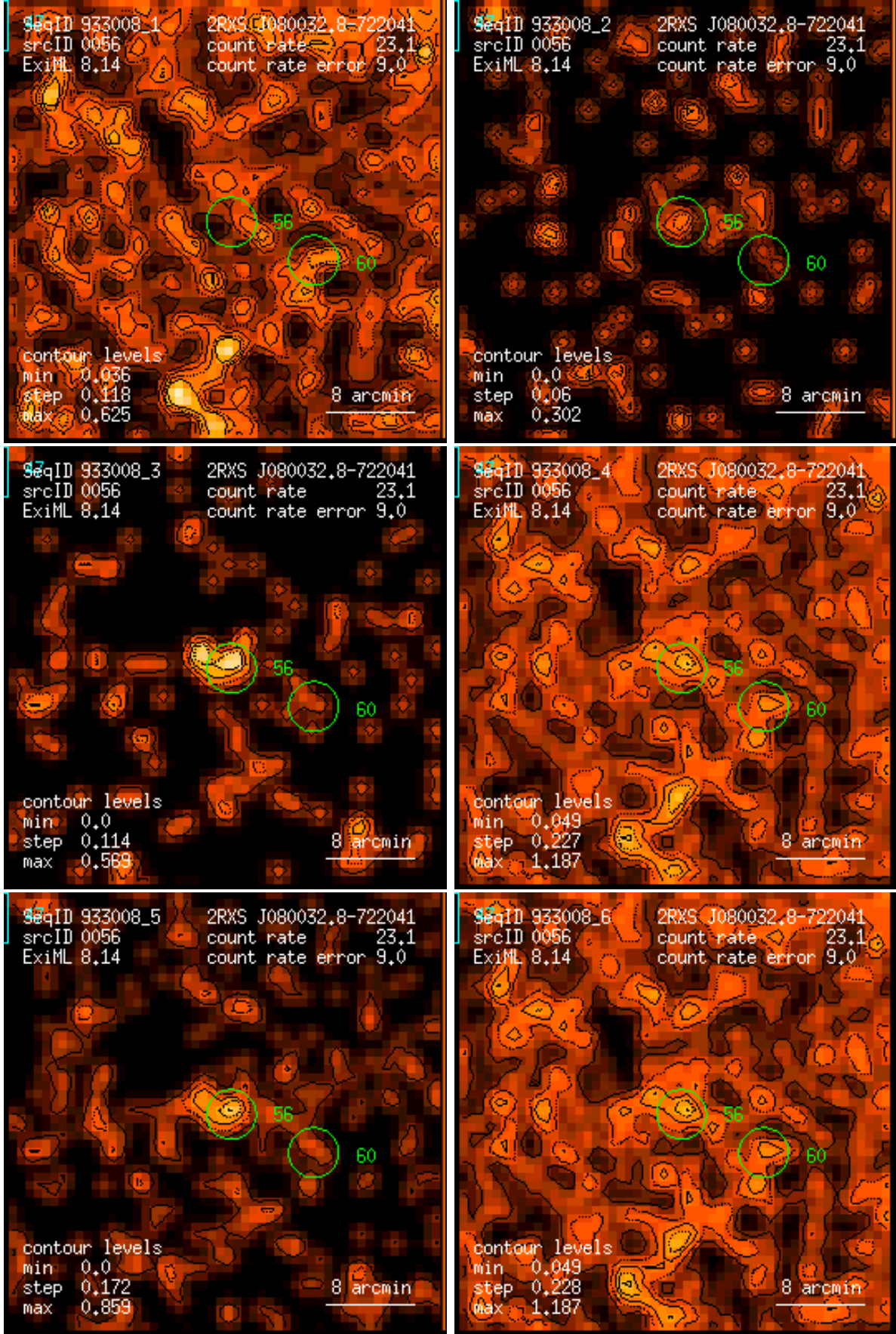
Figure 56: RASS 933008: detection 0056: band rate images, Gaussian filter: (1) PSPC channels 11 – 41, (2) 52 – 90, (3) 91 – 201, (4) 11 – 235, (5) 52 – 201, (6) 11 – 201. Broad band rates in counts/ks. Band rate contour levels in counts/ks/arcmin 2 .
